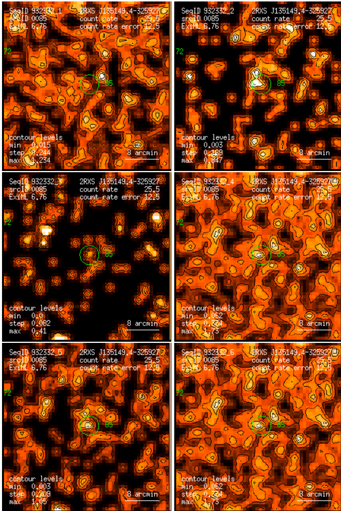
Figure 85: RASS 932332: detection 0085: band rate images, Gaussian filter: (1) PSPC channels 11 – 41, (2) 52 – 90, (3) 91 – 201, (4) 11 – 235, (5) 52 – 201, (6) 11 – 201. Broad band rates in counts/ks. Band rate contour levels in counts/ks/arcmin 2 .
