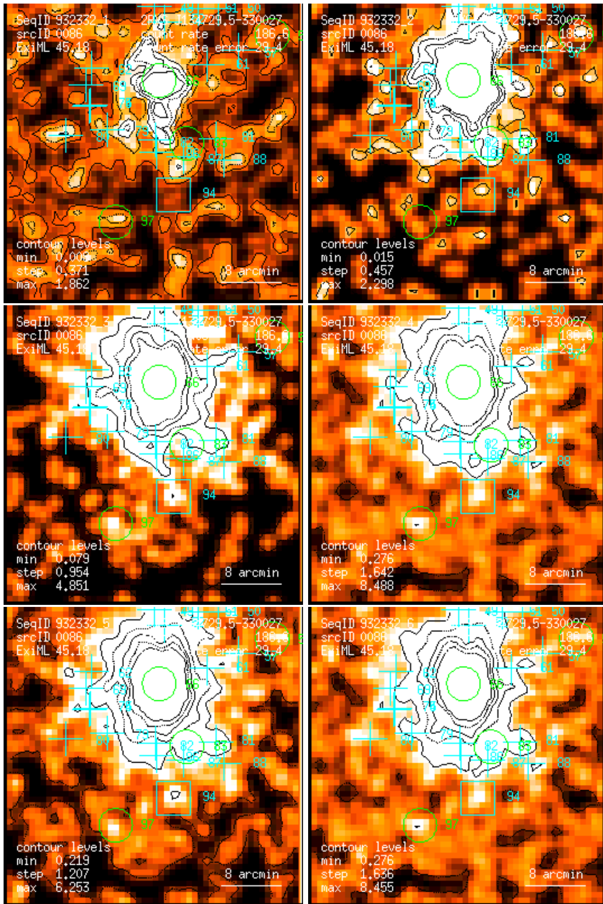
Figure 86: RASS 932332: detection 0086: band rate images, Gaussian filter: (1) PSPC channels 11 – 41, (2) 52 – 90, (3) 91 – 201, (4) 11 – 235, (5) 52 – 201, (6) 11 – 201. Broad band rates in counts/ks. Band rate contour levels in counts/ks/arcmin 2 .
