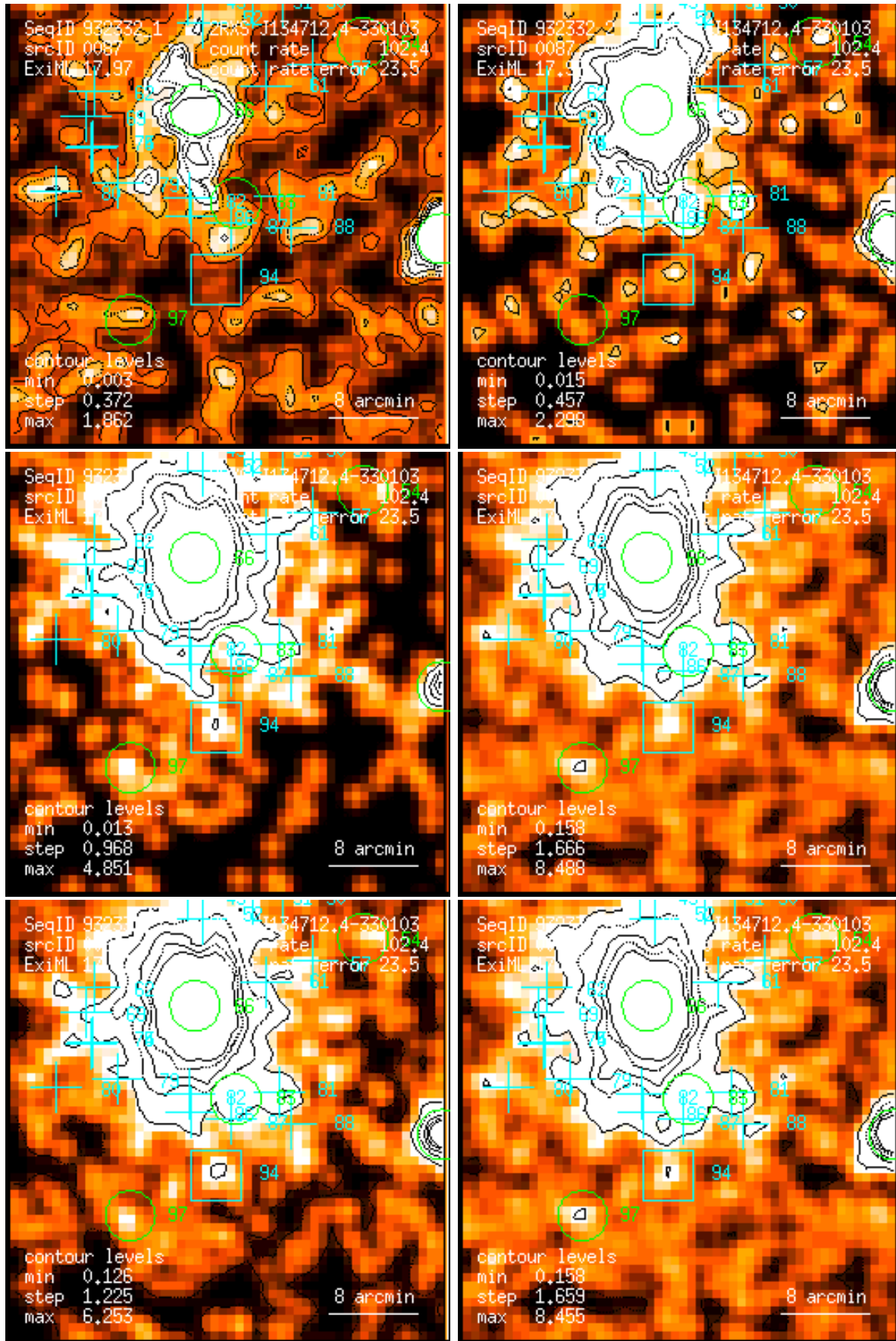
Figure 87: RASS 932332: detection 0087: band rate images, Gaussian filter: (1) PSPC channels 11 – 41, (2) 52 – 90, (3) 91 – 201, (4) 11 – 235, (5) 52 – 201, (6) 11 – 201. Broad band rates in counts/ks. Band rate contour levels in counts/ks/arcmin 2 .
