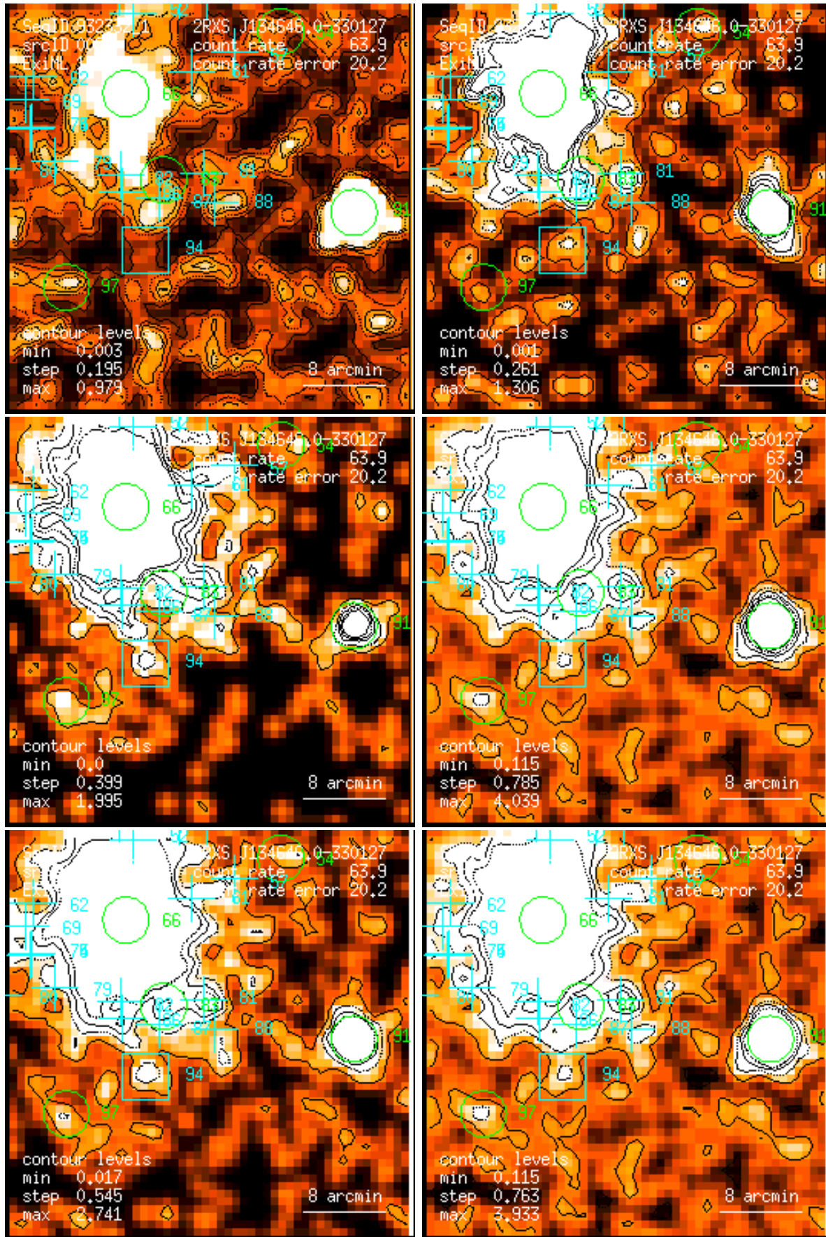
Figure 88: RASS 932332: detection 0088: band rate images, Gaussian filter: (1) PSPC channels 11 – 41, (2) 52 – 90, (3) 91 – 201, (4) 11 – 235, (5) 52 – 201, (6) 11 – 201. Broad band rates in counts/ks. Band rate contour levels in counts/ks/arcmin 2 .
