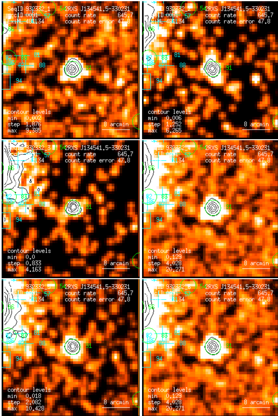
Figure 91: RASS 932332: detection 0091: band rate images, Gaussian filter: (1) PSPC channels 11 – 41, (2) 52 – 90, (3) 91 – 201, (4) 11 – 235, (5) 52 – 201, (6) 11 – 201. Broad band rates in counts/ks. Band rate contour levels in counts/ks/arcmin 2 .
