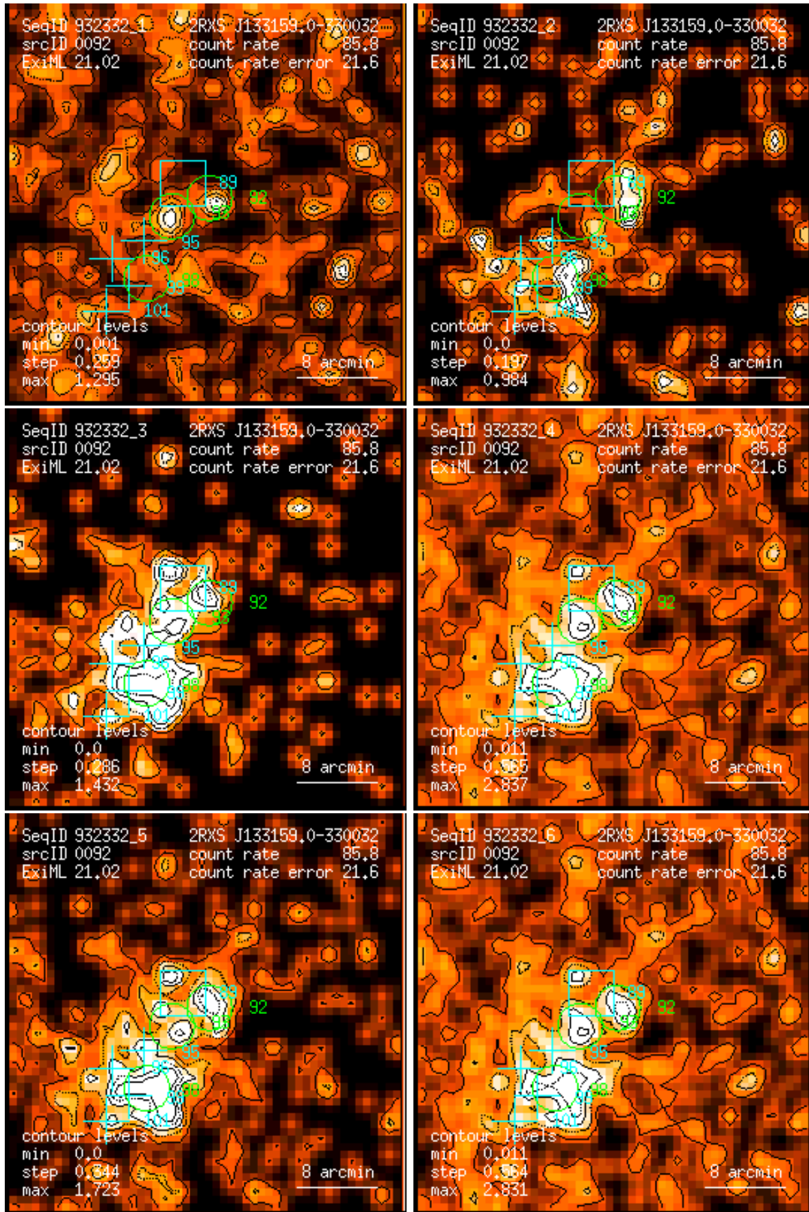
Figure 92: RASS 932332: detection 0092: band rate images, Gaussian filter: (1) PSPC channels 11 – 41, (2) 52 – 90, (3) 91 – 201, (4) 11 – 235, (5) 52 – 201, (6) 11 – 201. Broad band rates in counts/ks. Band rate contour levels in counts/ks/arcmin 2 .
