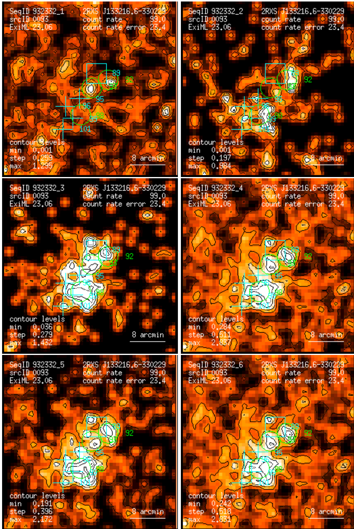
Figure 93: RASS 932332: detection 0093: band rate images, Gaussian filter: (1) PSPC channels 11 – 41, (2) 52 – 90, (3) 91 – 201, (4) 11 – 235, (5) 52 – 201, (6) 11 – 201. Broad band rates in counts/ks. Band rate contour levels in counts/ks/arcmin 2 .
