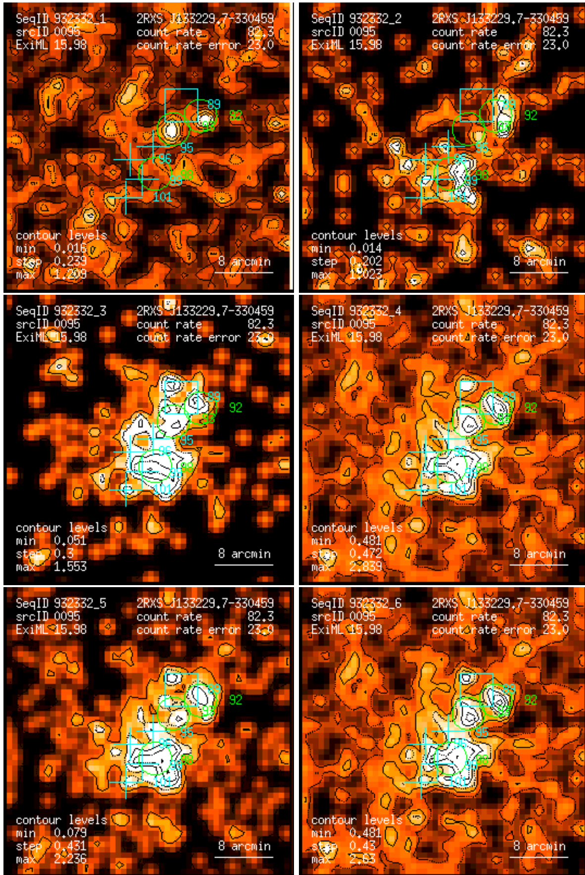
Figure 95: RASS 932332: detection 0095: band rate images, Gaussian filter: (1) PSPC channels 11 – 41, (2) 52 – 90, (3) 91 – 201, (4) 11 – 235, (5) 52 – 201, (6) 11 – 201. Broad band rates in counts/ks. Band rate contour levels in counts/ks/arcmin 2 .
