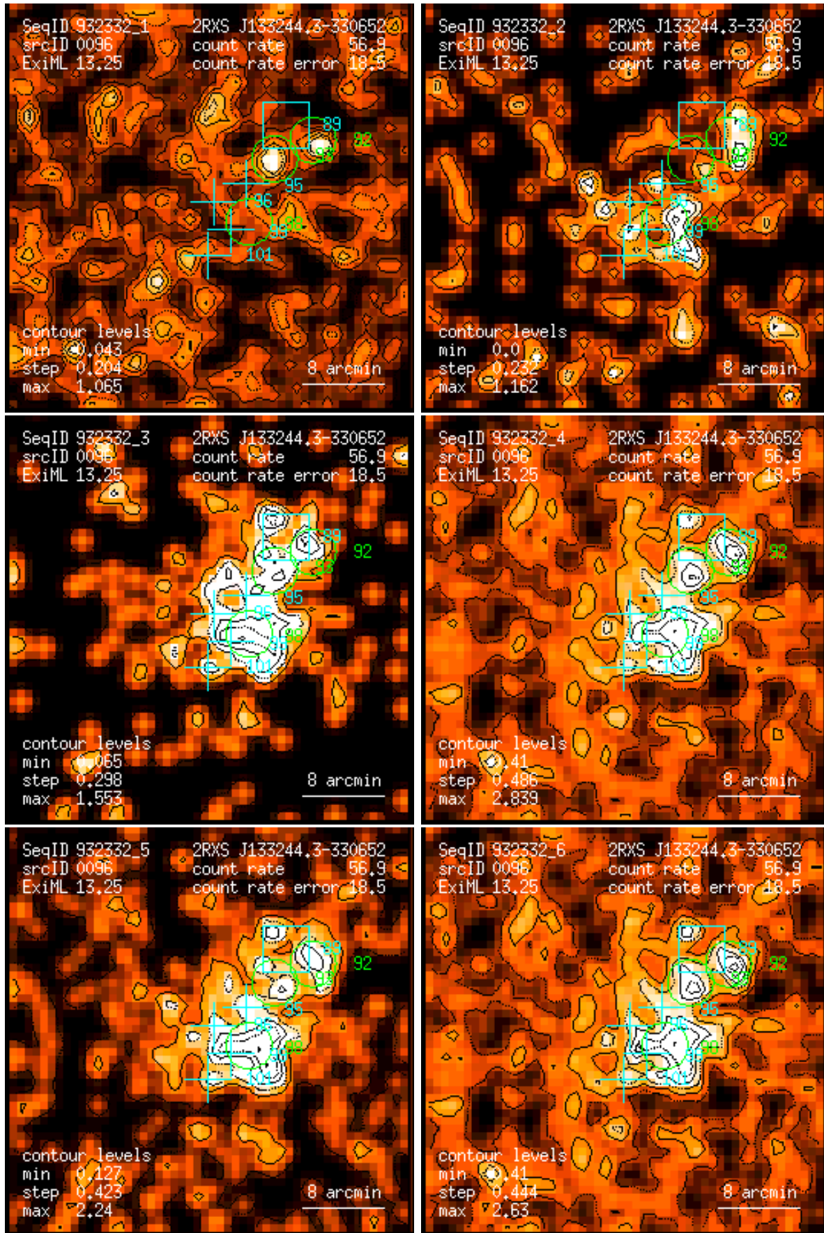
Figure 96: RASS 932332: detection 0096: band rate images, Gaussian filter: (1) PSPC channels 11 – 41, (2) 52 – 90, (3) 91 – 201, (4) 11 – 235, (5) 52 – 201, (6) 11 – 201. Broad band rates in counts/ks. Band rate contour levels in counts/ks/arcmin 2 .
