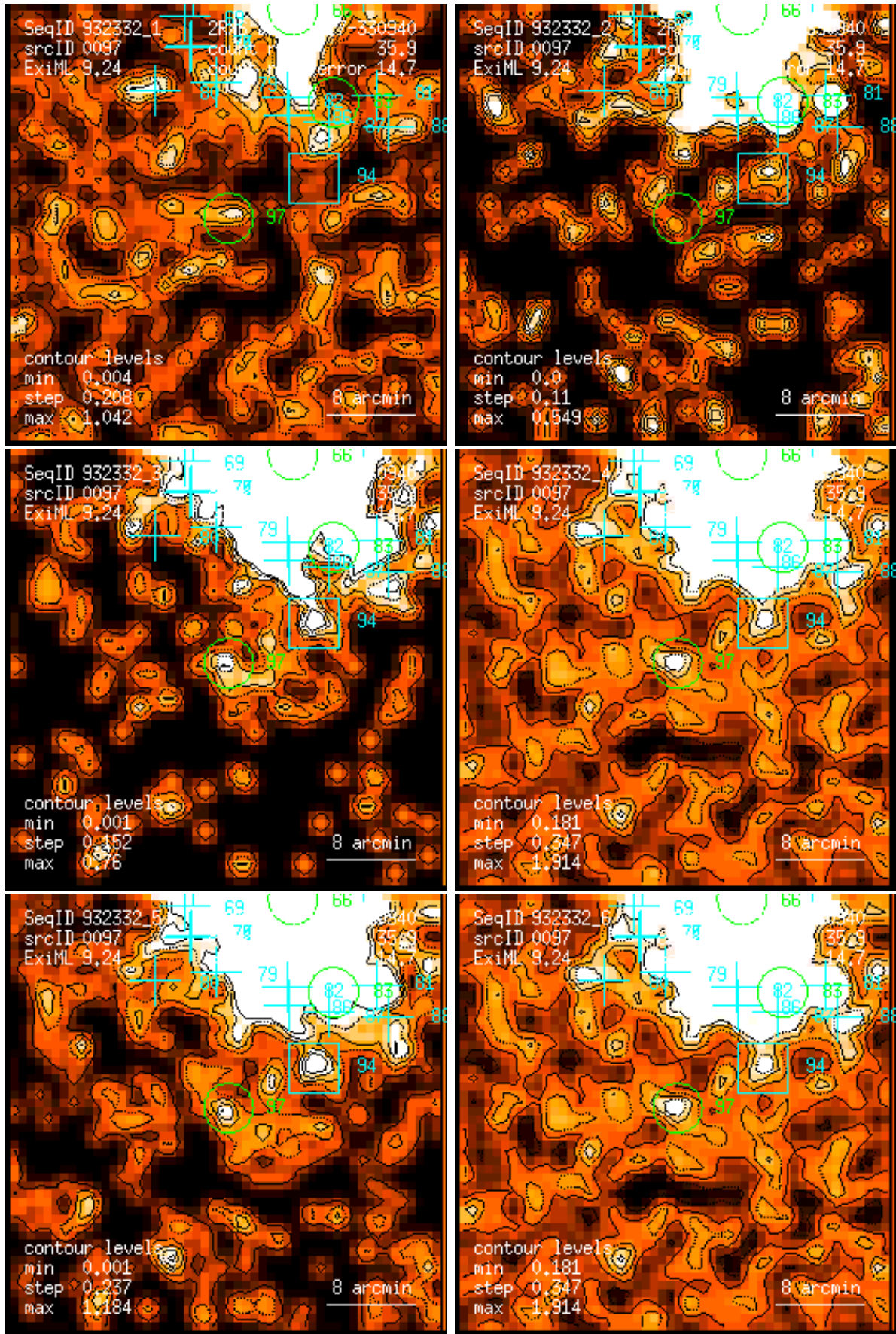
Figure 97: RASS 932332: detection 0097: band rate images, Gaussian filter: (1) PSPC channels 11 – 41, (2) 52 – 90, (3) 91 – 201, (4) 11 – 235, (5) 52 – 201, (6) 11 – 201. Broad band rates in counts/ks. Band rate contour levels in counts/ks/arcmin 2 .
