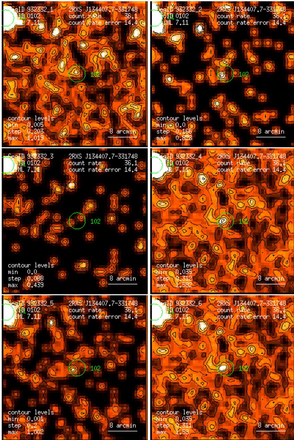
Figure 102: RASS 932332: detection 0102: band rate images, Gaussian filter: (1) PSPC channels 11 – 41, (2) 52 – 90, (3) 91 – 201, (4) 11 – 235, (5) 52 – 201, (6) 11 – 201. Broad band rates in counts/ks. Band rate contour levels in counts/ks/arcmin 2 .
