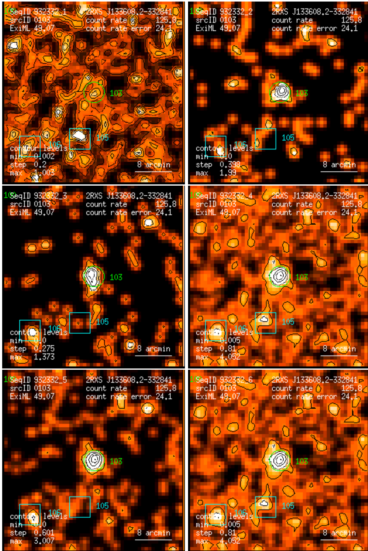
Figure 103: RASS 932332: detection 0103: band rate images, Gaussian filter: (1) PSPC channels 11 – 41, (2) 52 – 90, (3) 91 – 201, (4) 11 – 235, (5) 52 – 201, (6) 11 – 201. Broad band rates in counts/ks. Band rate contour levels in counts/ks/arcmin 2 .
