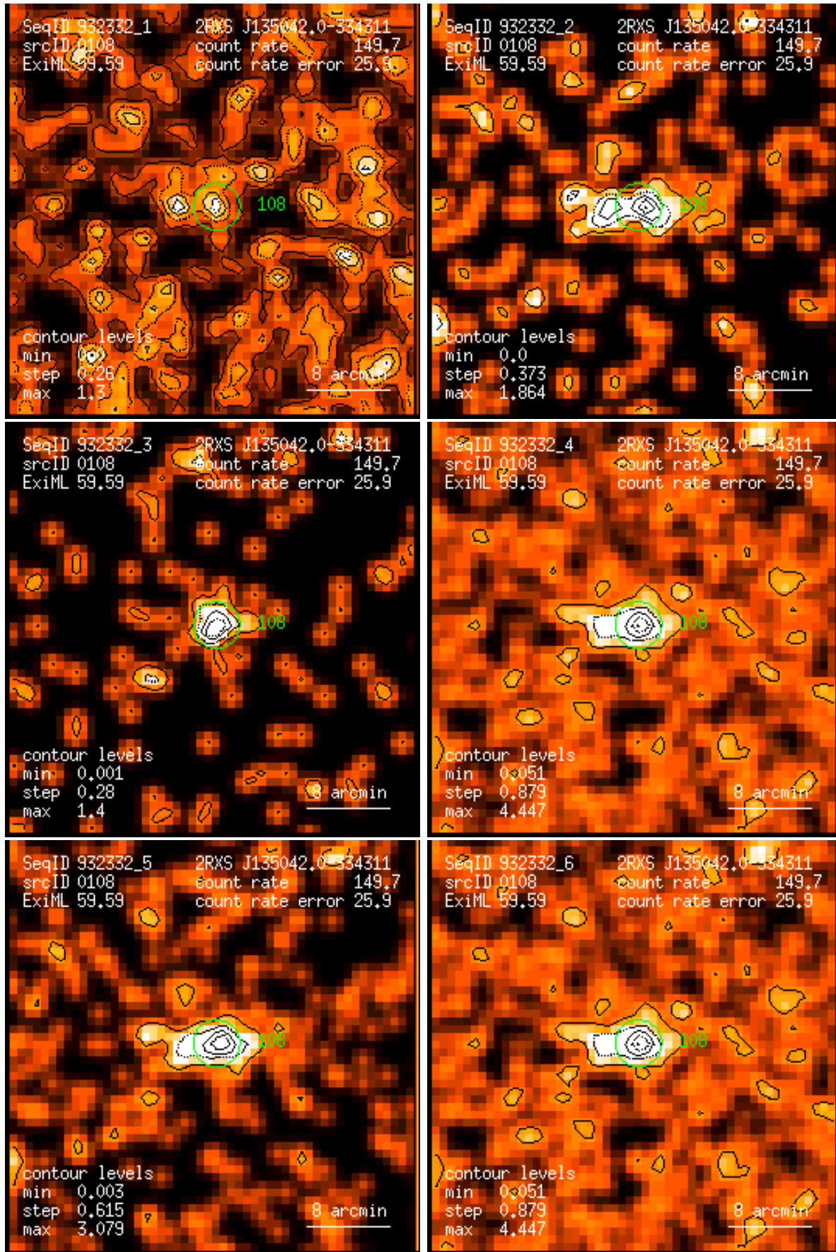
Figure 108: RASS 932332: detection 0108: band rate images, Gaussian filter: (1) PSPC channels 11 – 41, (2) 52 – 90, (3) 91 – 201, (4) 11 – 235, (5) 52 – 201, (6) 11 – 201. Broad band rates in counts/ks. Band rate contour levels in counts/ks/arcmin 2 .
