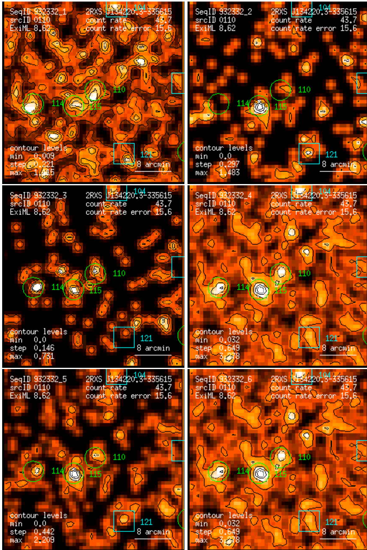
Figure 110: RASS 932332: detection 0110: band rate images, Gaussian filter: (1) PSPC channels 11 – 41, (2) 52 – 90, (3) 91 – 201, (4) 11 – 235, (5) 52 – 201, (6) 11 – 201. Broad band rates in counts/ks. Band rate contour levels in counts/ks/arcmin 2 .
