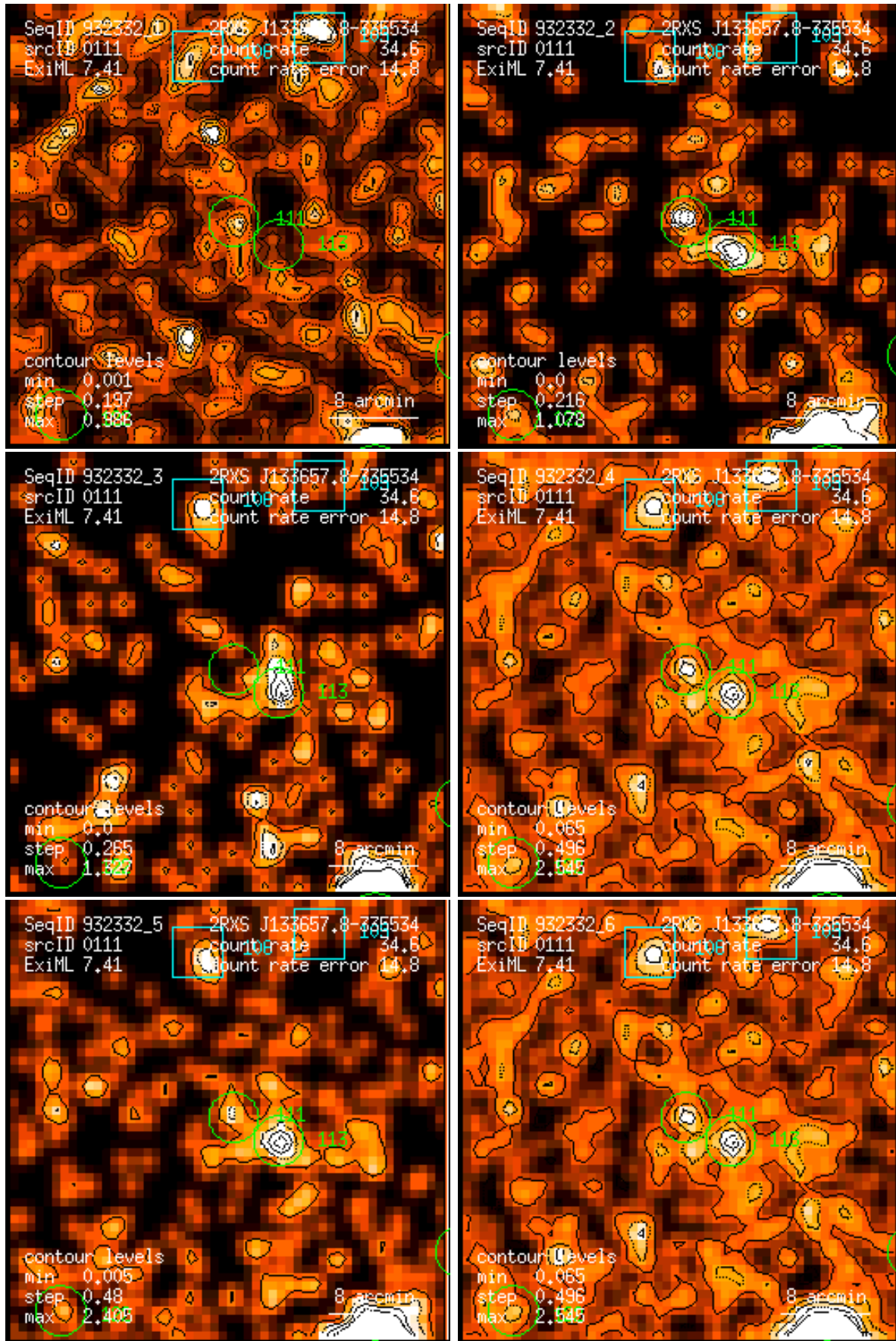
Figure 111: RASS 932332: detection 0111: band rate images, Gaussian filter: (1) PSPC channels 11 – 41, (2) 52 – 90, (3) 91 – 201, (4) 11 – 235, (5) 52 – 201, (6) 11 – 201. Broad band rates in counts/ks. Band rate contour levels in counts/ks/arcmin 2 .
