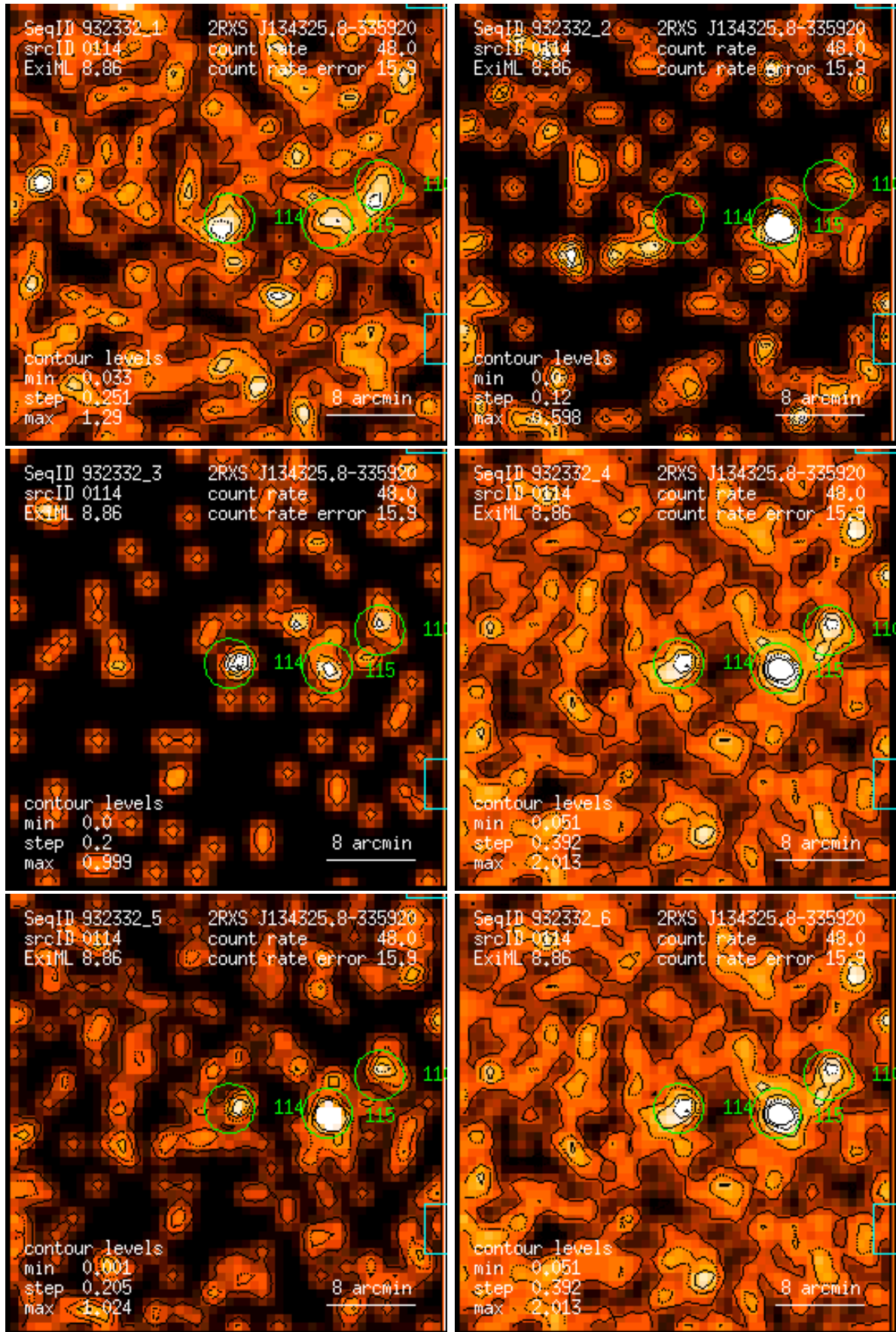
Figure 114: RASS 932332: detection 0114: band rate images, Gaussian filter: (1) PSPC channels 11 – 41, (2) 52 – 90, (3) 91 – 201, (4) 11 – 235, (5) 52 – 201, (6) 11 – 201. Broad band rates in counts/ks. Band rate contour levels in counts/ks/arcmin 2 .
