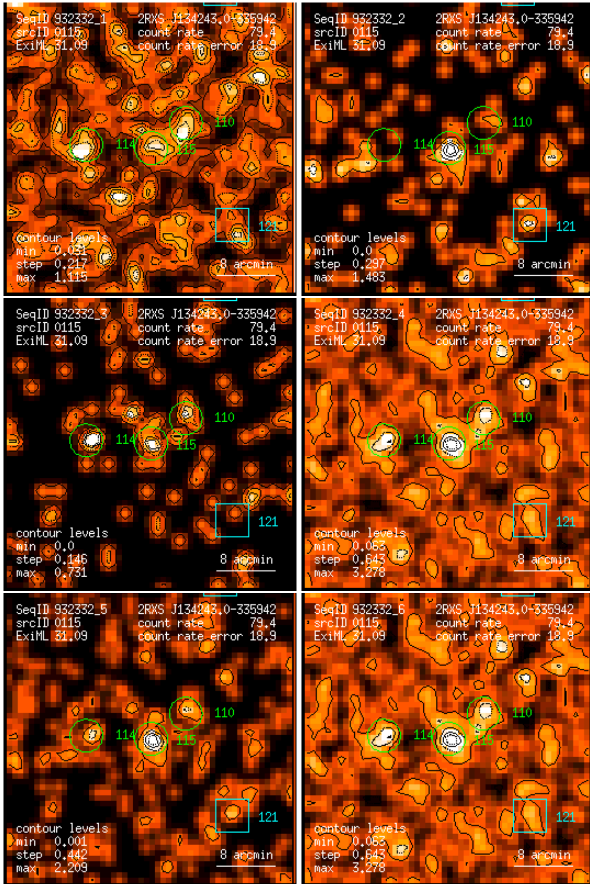
Figure 115: RASS 932332: detection 0115: band rate images, Gaussian filter: (1) PSPC channels 11 – 41, (2) 52 – 90, (3) 91 – 201, (4) 11 – 235, (5) 52 – 201, (6) 11 – 201. Broad band rates in counts/ks. Band rate contour levels in counts/ks/arcmin 2 .
