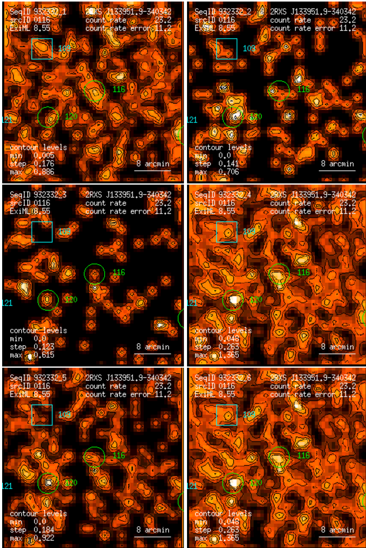
Figure 116: RASS 932332: detection 0116: band rate images, Gaussian filter: (1) PSPC channels 11 – 41, (2) 52 – 90, (3) 91 – 201, (4) 11 – 235, (5) 52 – 201, (6) 11 – 201. Broad band rates in counts/ks. Band rate contour levels in counts/ks/arcmin 2 .
