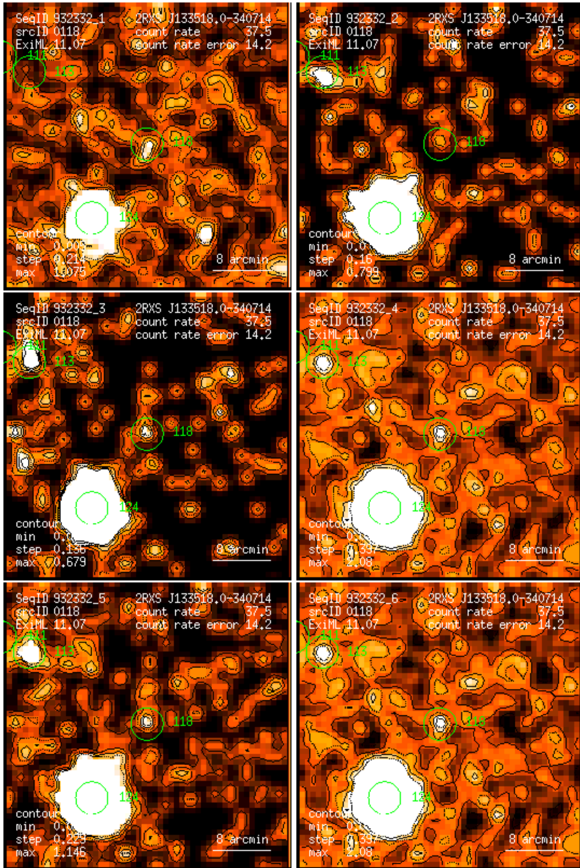
Figure 118: RASS 932332: detection 0118: band rate images, Gaussian filter: (1) PSPC channels 11 – 41, (2) 52 – 90, (3) 91 – 201, (4) 11 – 235, (5) 52 – 201, (6) 11 – 201. Broad band rates in counts/ks. Band rate contour levels in counts/ks/arcmin 2 .
