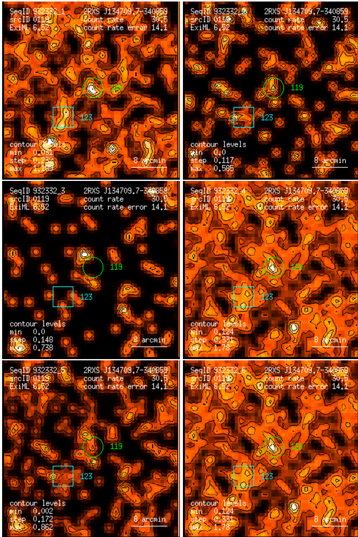
Figure 119: RASS 932332: detection 0119: band rate images, Gaussian filter: (1) PSPC channels 11 – 41, (2) 52 – 90, (3) 91 – 201, (4) 11 – 235, (5) 52 – 201, (6) 11 – 201. Broad band rates in counts/ks. Band rate contour levels in counts/ks/arcmin 2 .
