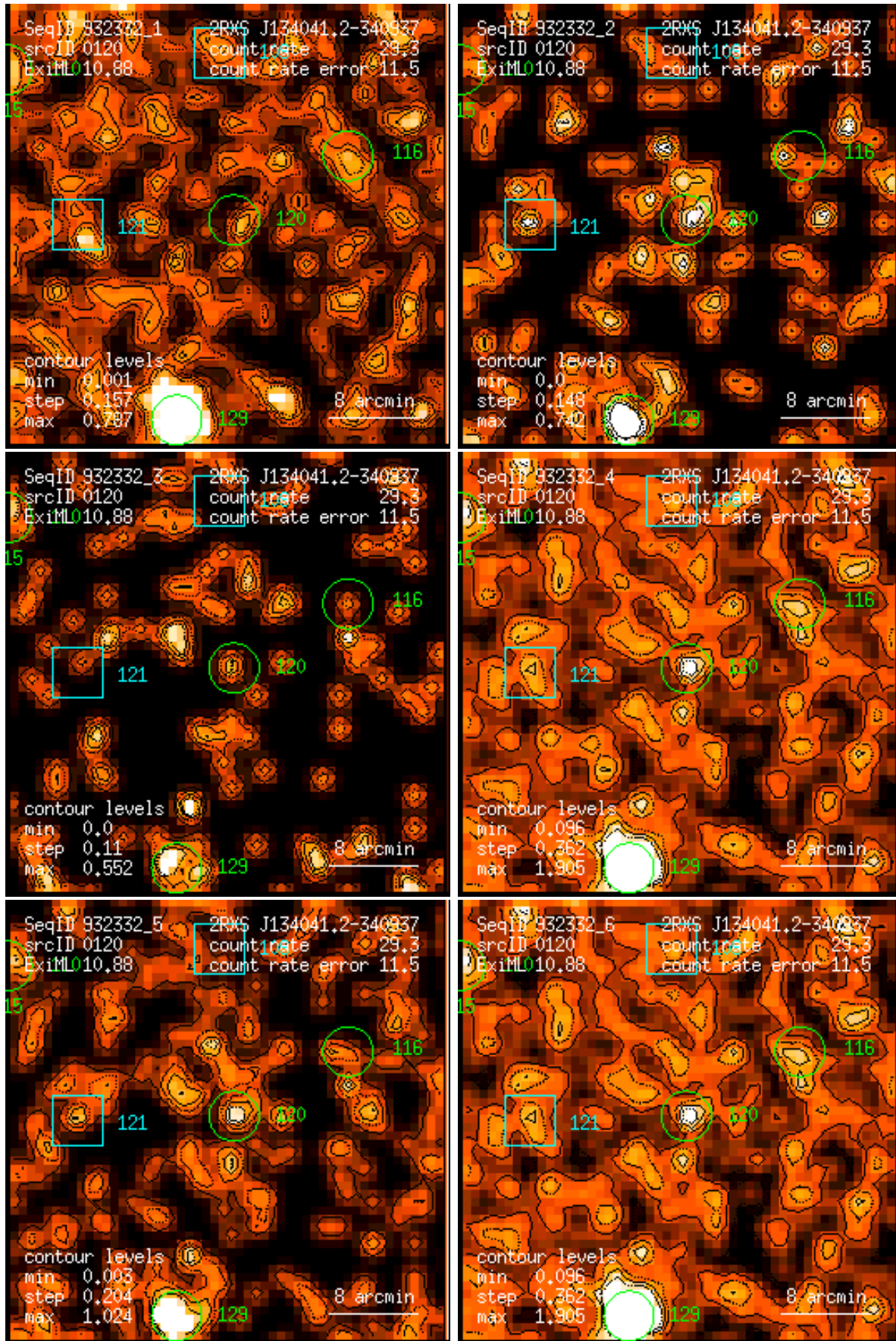
Figure 120: RASS 932332: detection 0120: band rate images, Gaussian filter: (1) PSPC channels 11 – 41, (2) 52 – 90, (3) 91 – 201, (4) 11 – 235, (5) 52 – 201, (6) 11 – 201. Broad band rates in counts/ks. Band rate contour levels in counts/ks/arcmin 2 .
