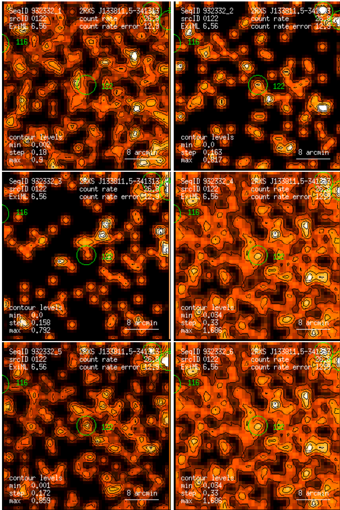
Figure 122: RASS 932332: detection 0122: band rate images, Gaussian filter: (1) PSPC channels 11 – 41, (2) 52 – 90, (3) 91 – 201, (4) 11 – 235, (5) 52 – 201, (6) 11 – 201. Broad band rates in counts/ks. Band rate contour levels in counts/ks/arcmin 2 .
