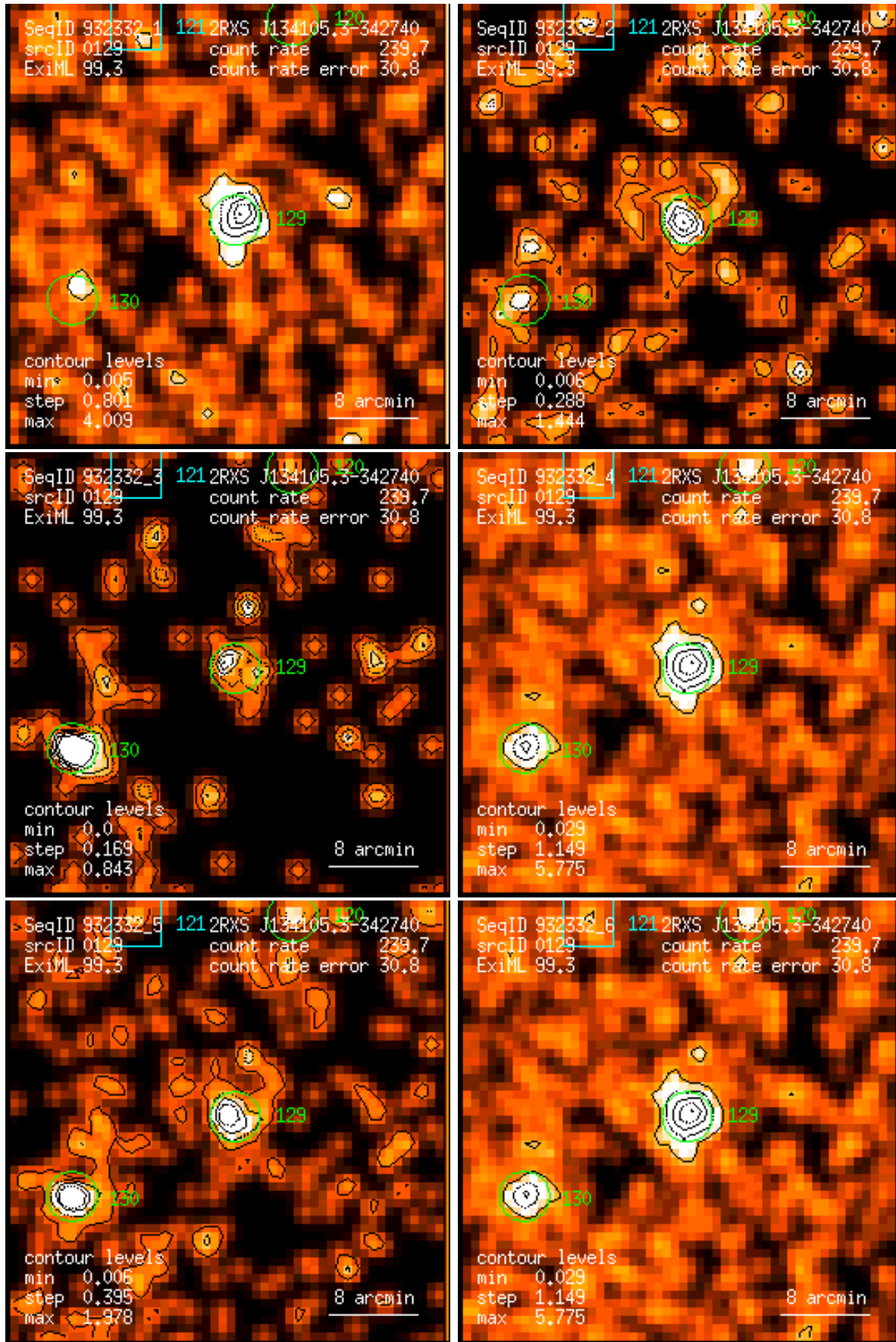
Figure 129: RASS 932332: detection 0129: band rate images, Gaussian filter: (1) PSPC channels 11 – 41, (2) 52 – 90, (3) 91 – 201, (4) 11 – 235, (5) 52 – 201, (6) 11 – 201. Broad band rates in counts/ks. Band rate contour levels in counts/ks/arcmin 2 .
