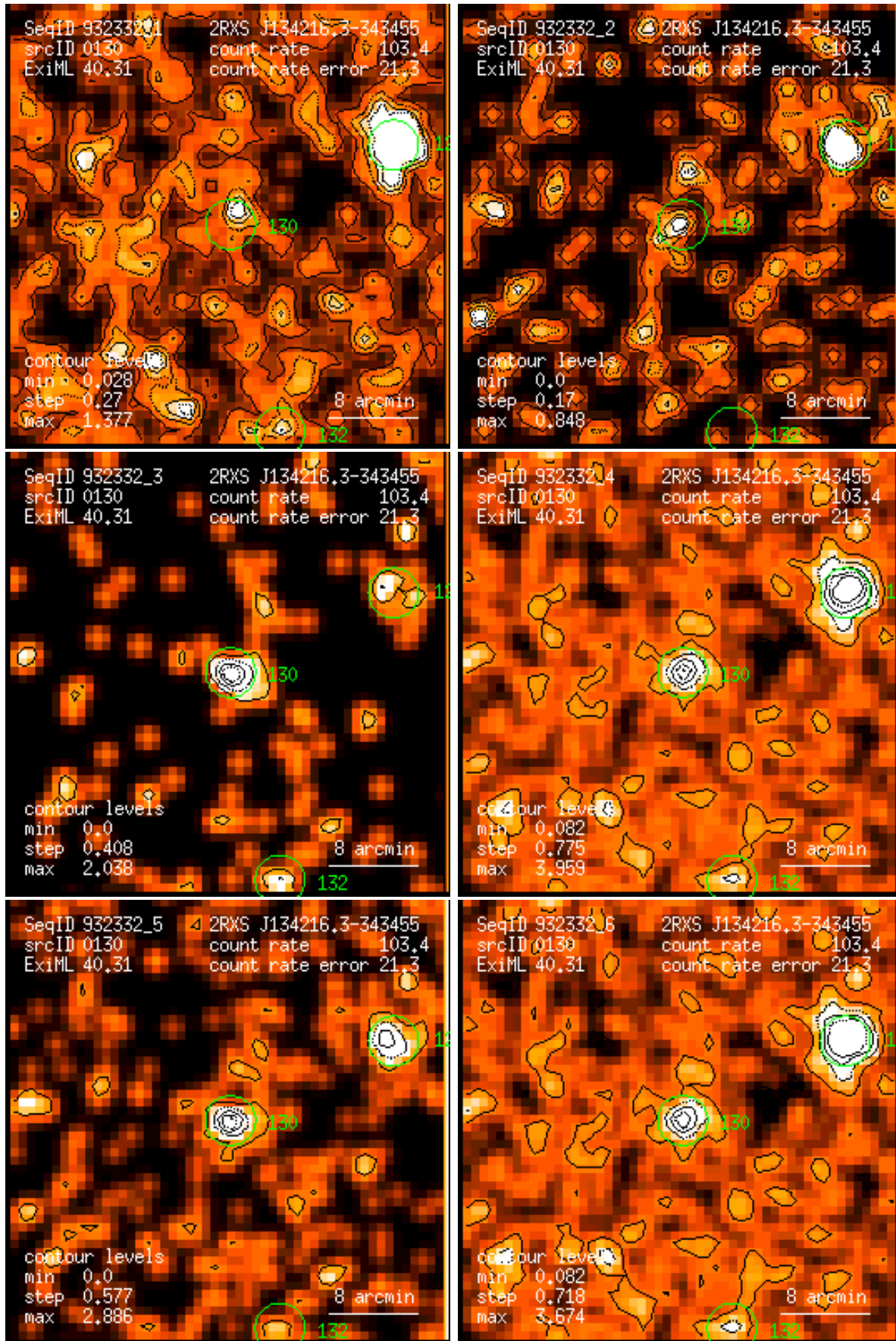
Figure 130: RASS 932332: detection 0130: band rate images, Gaussian filter: (1) PSPC channels 11 – 41, (2) 52 – 90, (3) 91 – 201, (4) 11 – 235, (5) 52 – 201, (6) 11 – 201. Broad band rates in counts/ks. Band rate contour levels in counts/ks/arcmin 2 .
