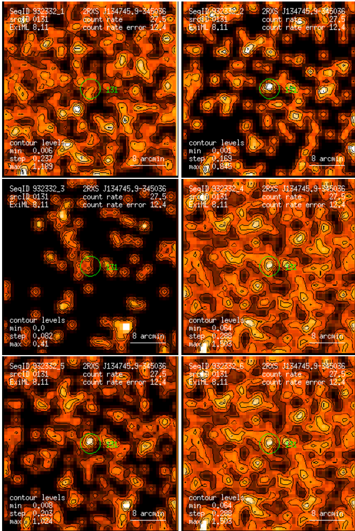
Figure 131: RASS 932332: detection 0131: band rate images, Gaussian filter: (1) PSPC channels 11 – 41, (2) 52 – 90, (3) 91 – 201, (4) 11 – 235, (5) 52 – 201, (6) 11 – 201. Broad band rates in counts/ks. Band rate contour levels in counts/ks/arcmin 2 .
