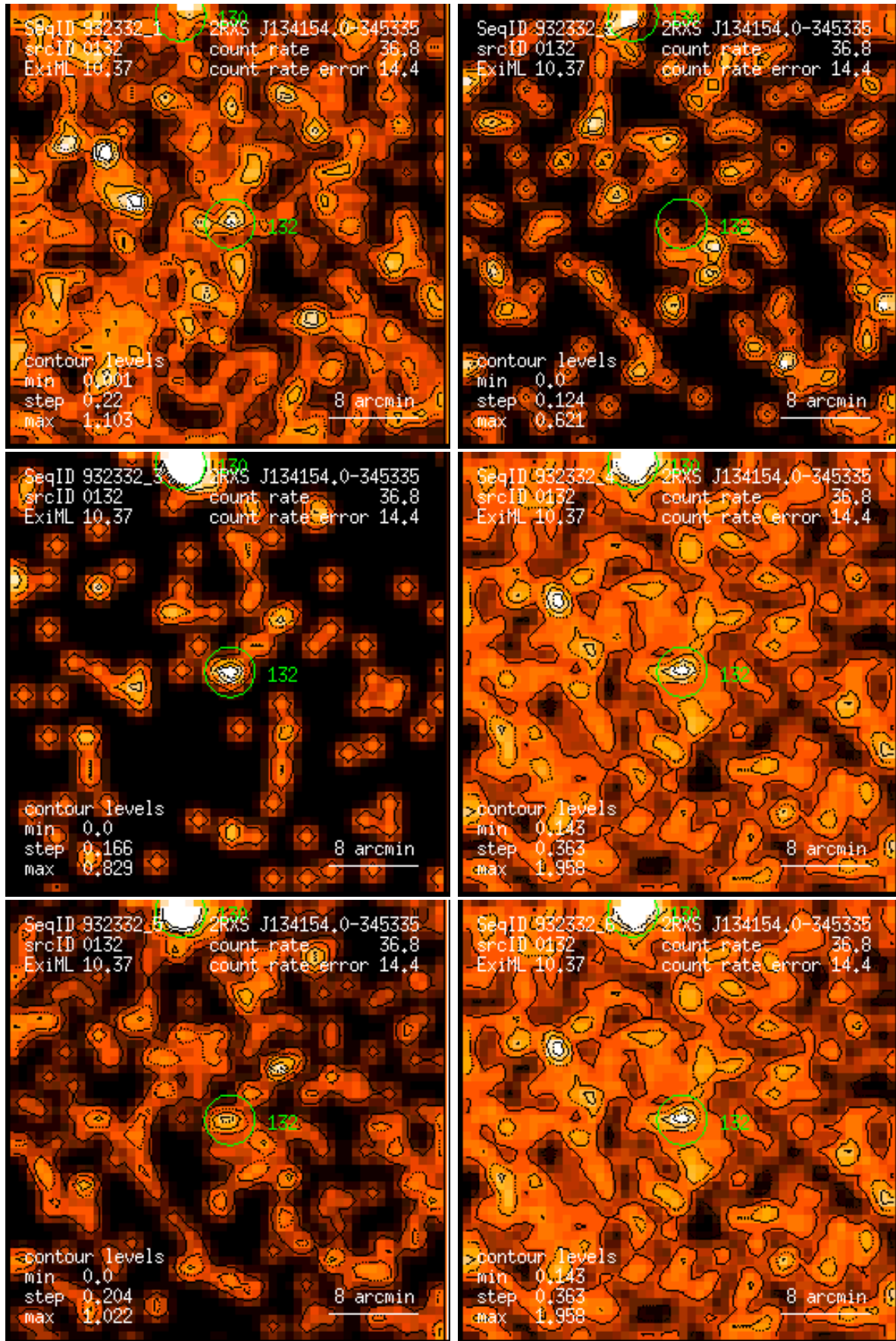
Figure 132: RASS 932332: detection 0132: band rate images, Gaussian filter: (1) PSPC channels 11 – 41, (2) 52 – 90, (3) 91 – 201, (4) 11 – 235, (5) 52 – 201, (6) 11 – 201. Broad band rates in counts/ks. Band rate contour levels in counts/ks/arcmin 2 .
