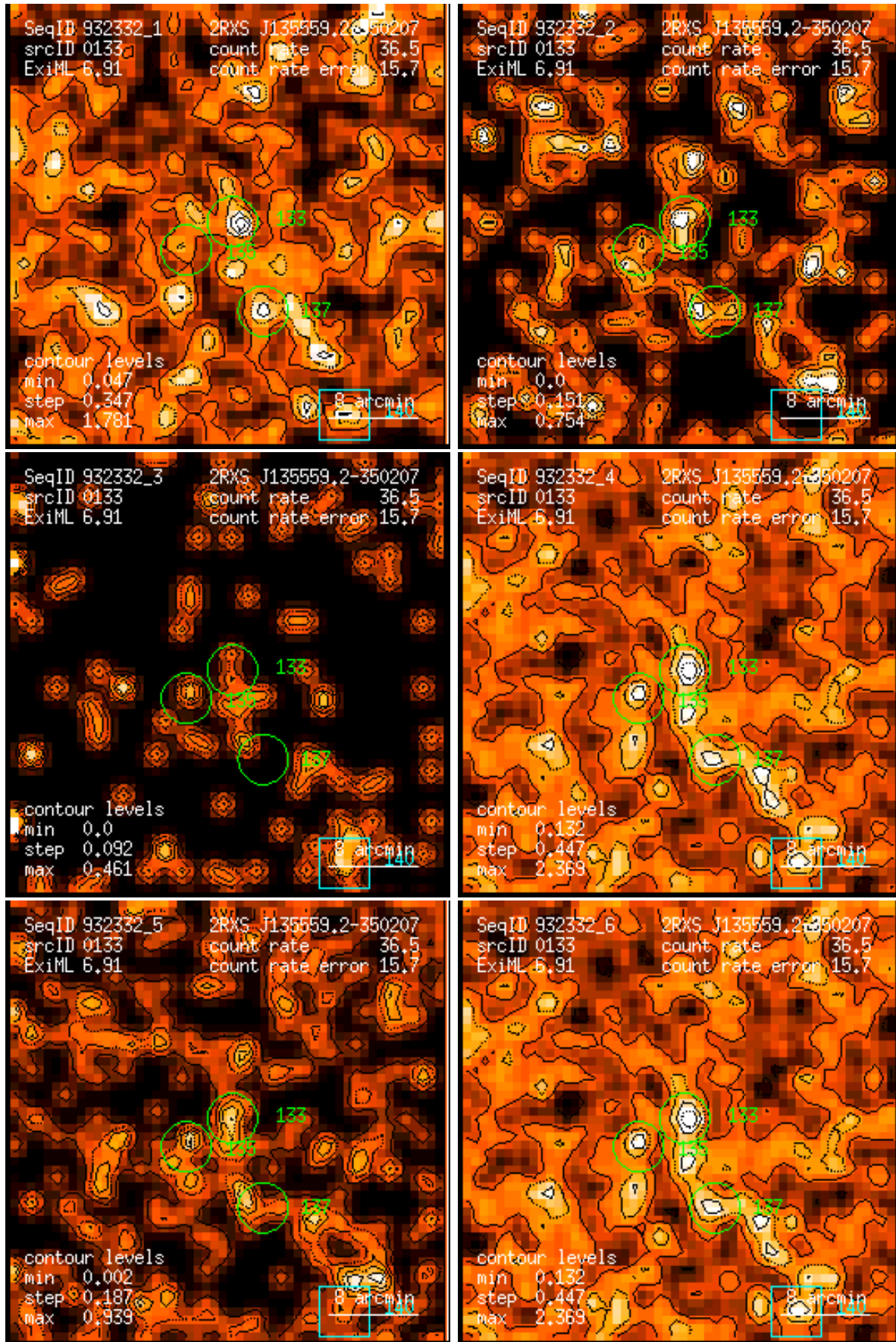
Figure 133: RASS 932332: detection 0133: band rate images, Gaussian filter: (1) PSPC channels 11 – 41, (2) 52 – 90, (3) 91 – 201, (4) 11 – 235, (5) 52 – 201, (6) 11 – 201. Broad band rates in counts/ks. Band rate contour levels in counts/ks/arcmin 2 .
