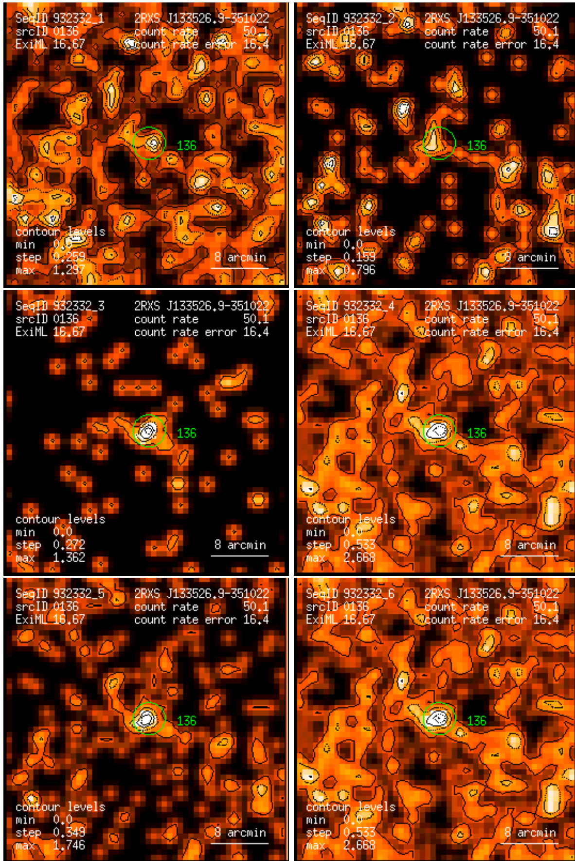
Figure 136: RASS 932332: detection 0136: band rate images, Gaussian filter: (1) PSPC channels 11 – 41, (2) 52 – 90, (3) 91 – 201, (4) 11 – 235, (5) 52 – 201, (6) 11 – 201. Broad band rates in counts/ks. Band rate contour levels in counts/ks/arcmin 2 .
