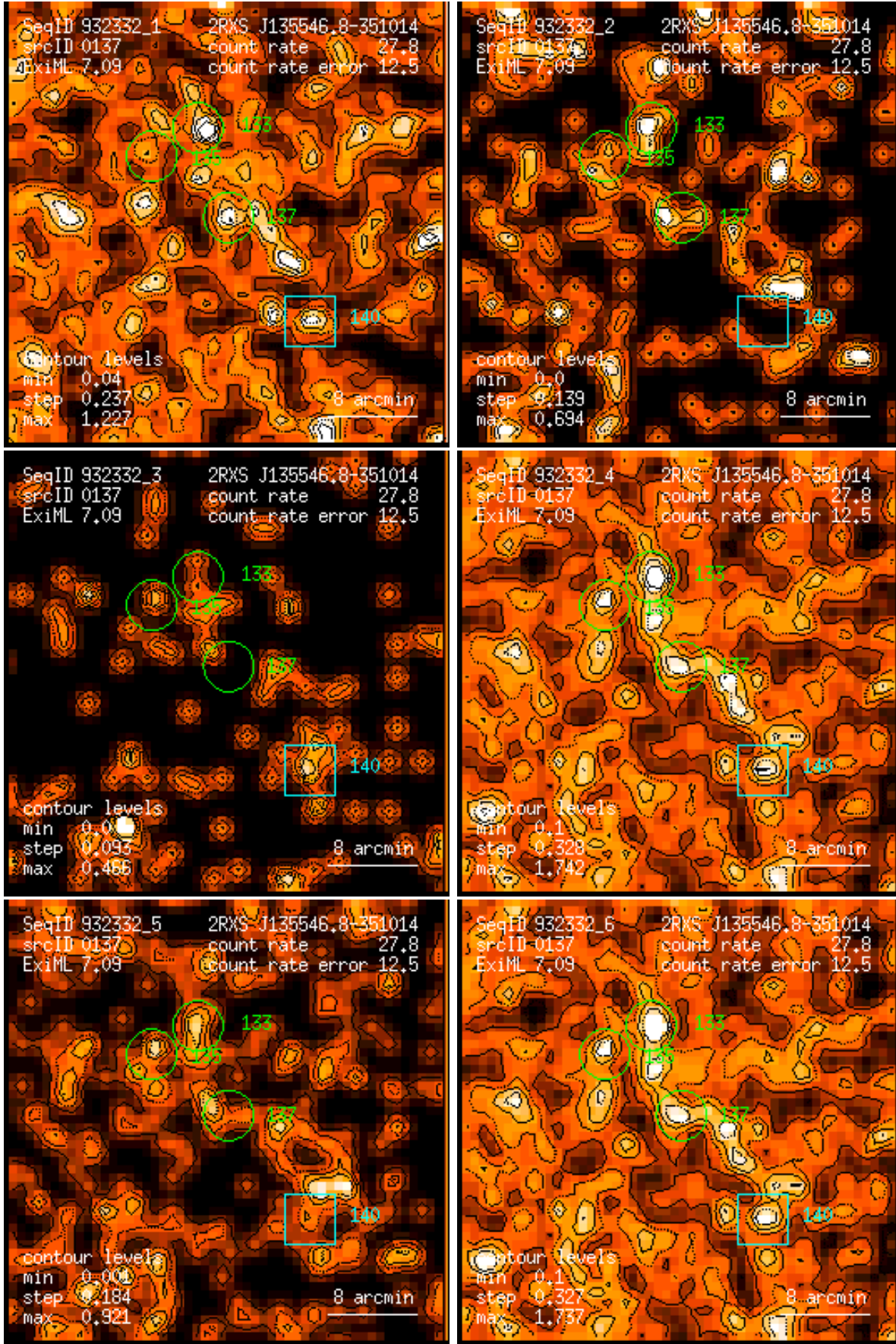
Figure 137: RASS 932332: detection 0137: band rate images, Gaussian filter: (1) PSPC channels 11 – 41, (2) 52 – 90, (3) 91 – 201, (4) 11 – 235, (5) 52 – 201, (6) 11 – 201. Broad band rates in counts/ks. Band rate contour levels in counts/ks/arcmin 2 .
