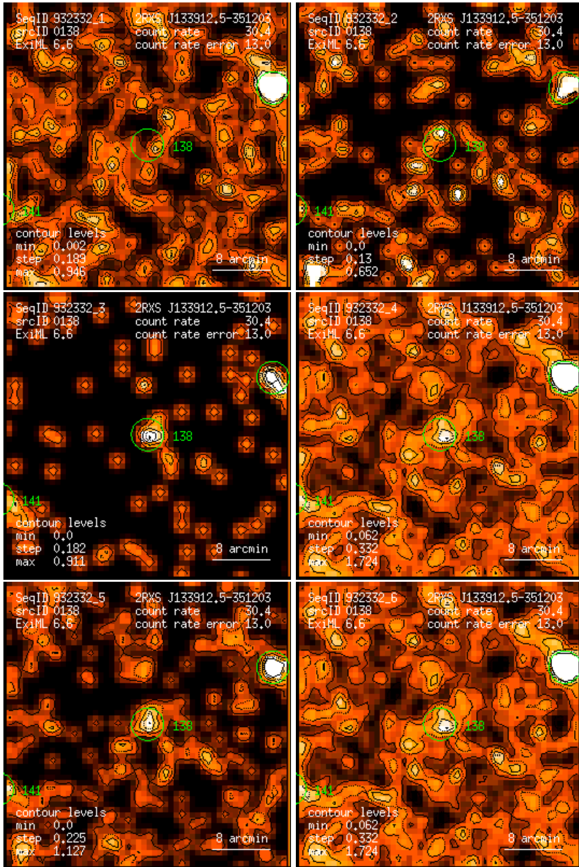
Figure 138: RASS 932332: detection 0138: band rate images, Gaussian filter: (1) PSPC channels 11 – 41, (2) 52 – 90, (3) 91 – 201, (4) 11 – 235, (5) 52 – 201, (6) 11 – 201. Broad band rates in counts/ks. Band rate contour levels in counts/ks/arcmin 2 .
