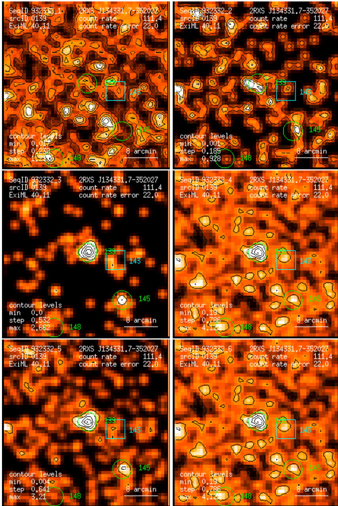
Figure 139: RASS 932332: detection 0139: band rate images, Gaussian filter: (1) PSPC channels 11 – 41, (2) 52 – 90, (3) 91 – 201, (4) 11 – 235, (5) 52 – 201, (6) 11 – 201. Broad band rates in counts/ks. Band rate contour levels in counts/ks/arcmin 2 .
