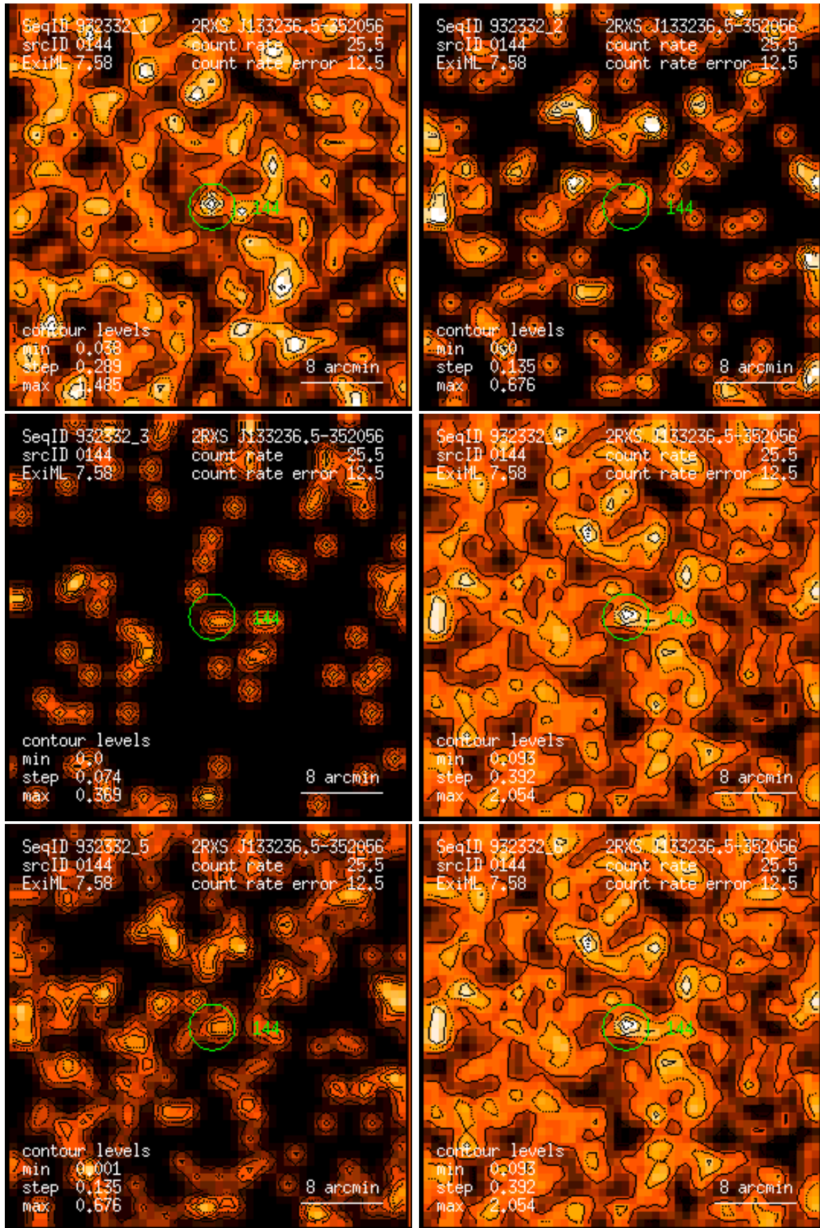
Figure 144: RASS 932332: detection 0144: band rate images, Gaussian filter: (1) PSPC channels 11 – 41, (2) 52 – 90, (3) 91 – 201, (4) 11 – 235, (5) 52 – 201, (6) 11 – 201. Broad band rates in counts/ks. Band rate contour levels in counts/ks/arcmin 2 .
