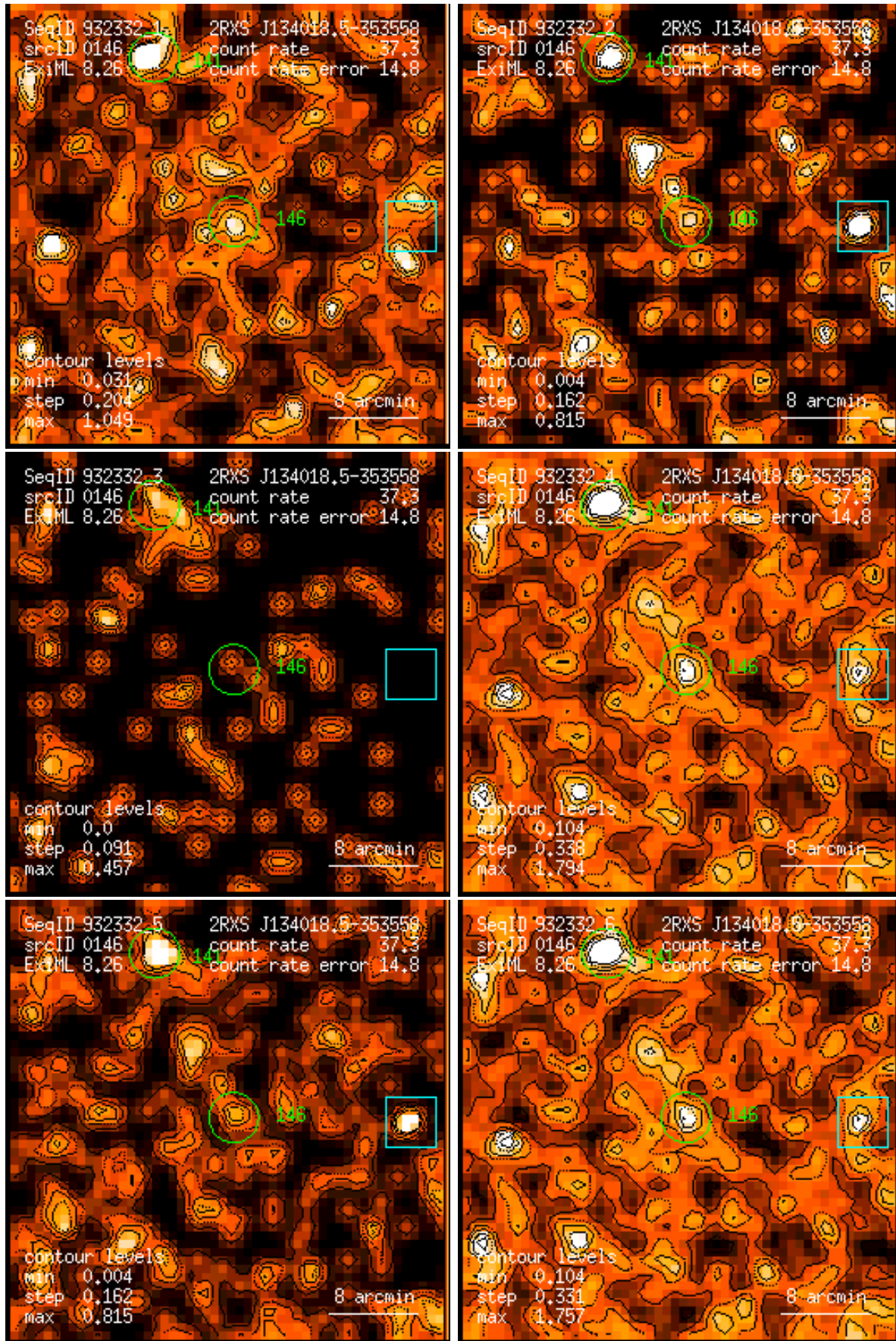
Figure 146: RASS 932332: detection 0146: band rate images, Gaussian filter: (1) PSPC channels 11 – 41, (2) 52 – 90, (3) 91 – 201, (4) 11 – 235, (5) 52 – 201, (6) 11 – 201. Broad band rates in counts/ks. Band rate contour levels in counts/ks/arcmin 2 .
