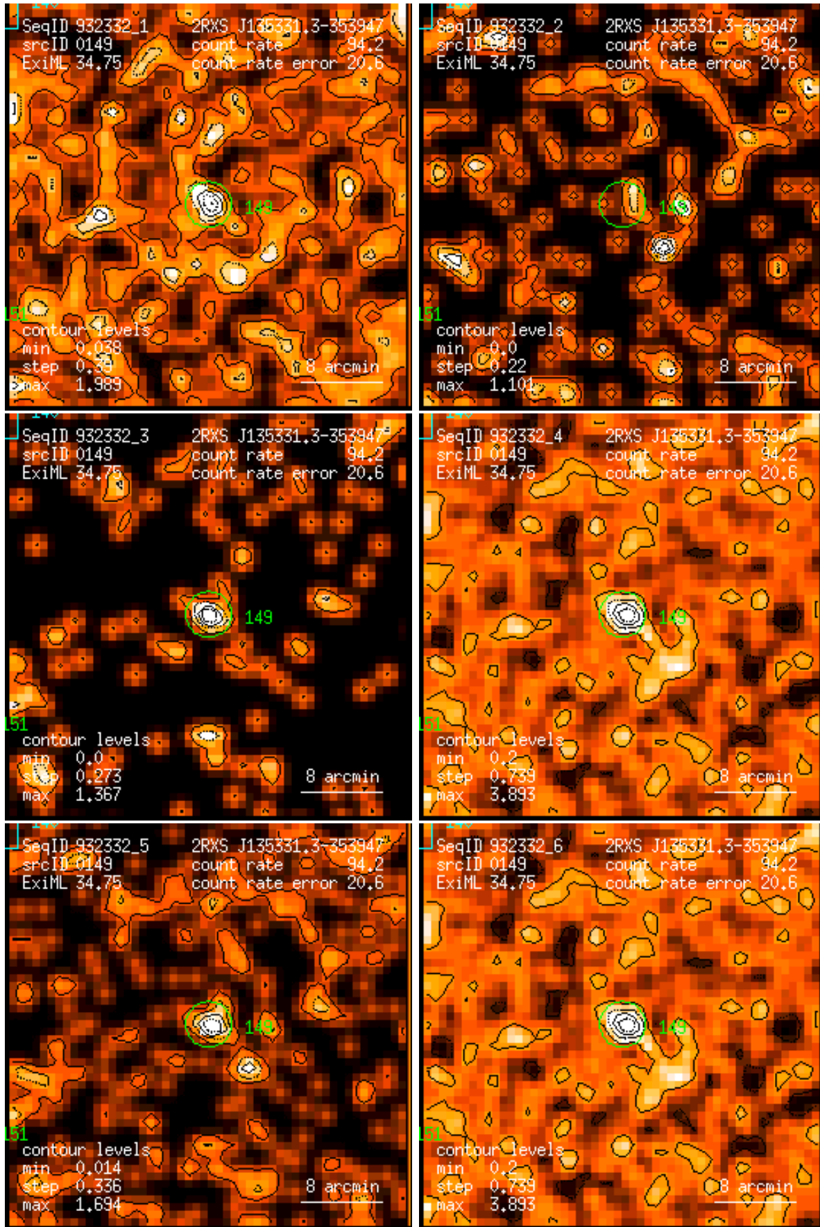
Figure 149: RASS 932332: detection 0149: band rate images, Gaussian filter: (1) PSPC channels 11 – 41, (2) 52 – 90, (3) 91 – 201, (4) 11 – 235, (5) 52 – 201, (6) 11 – 201. Broad band rates in counts/ks. Band rate contour levels in counts/ks/arcmin 2 .
