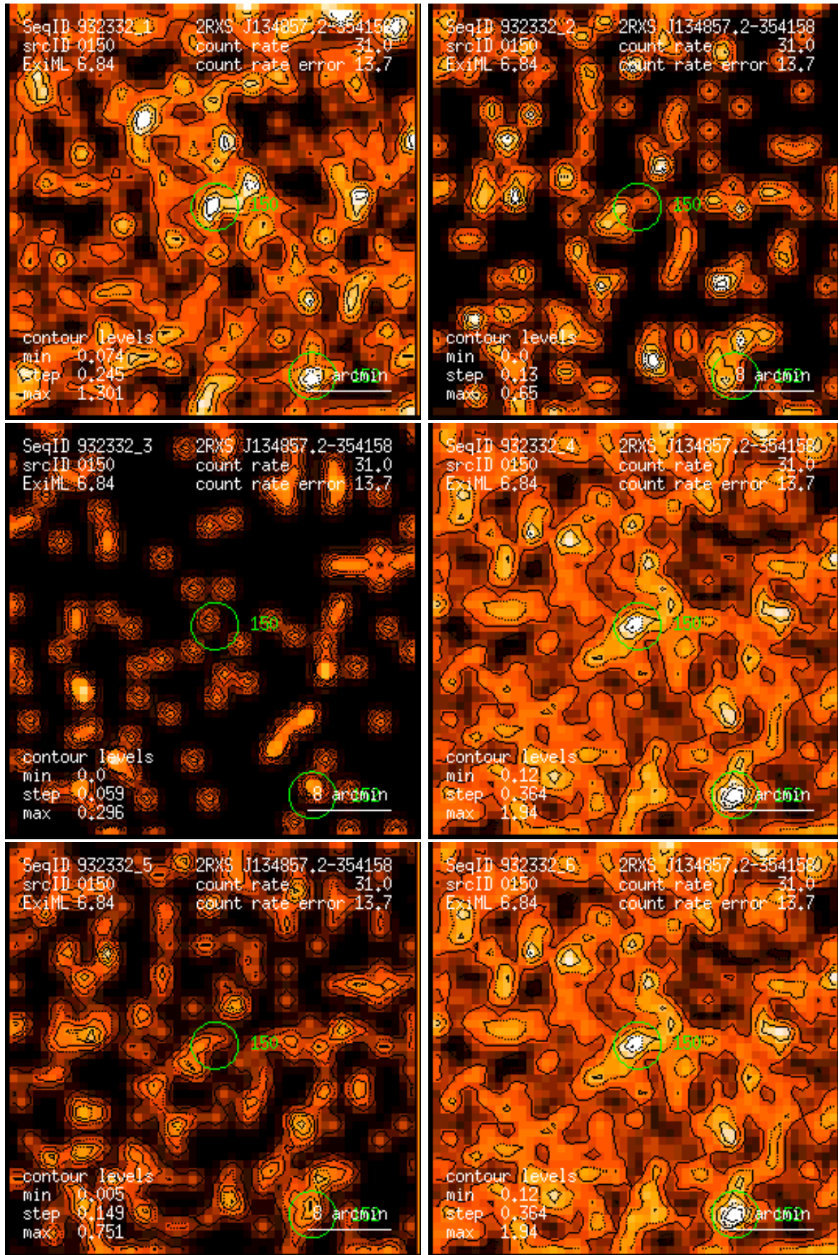
Figure 150: RASS 932332: detection 0150: band rate images, Gaussian filter: (1) PSPC channels 11 – 41, (2) 52 – 90, (3) 91 – 201, (4) 11 – 235, (5) 52 – 201, (6) 11 – 201. Broad band rates in counts/ks. Band rate contour levels in counts/ks/arcmin 2 .
