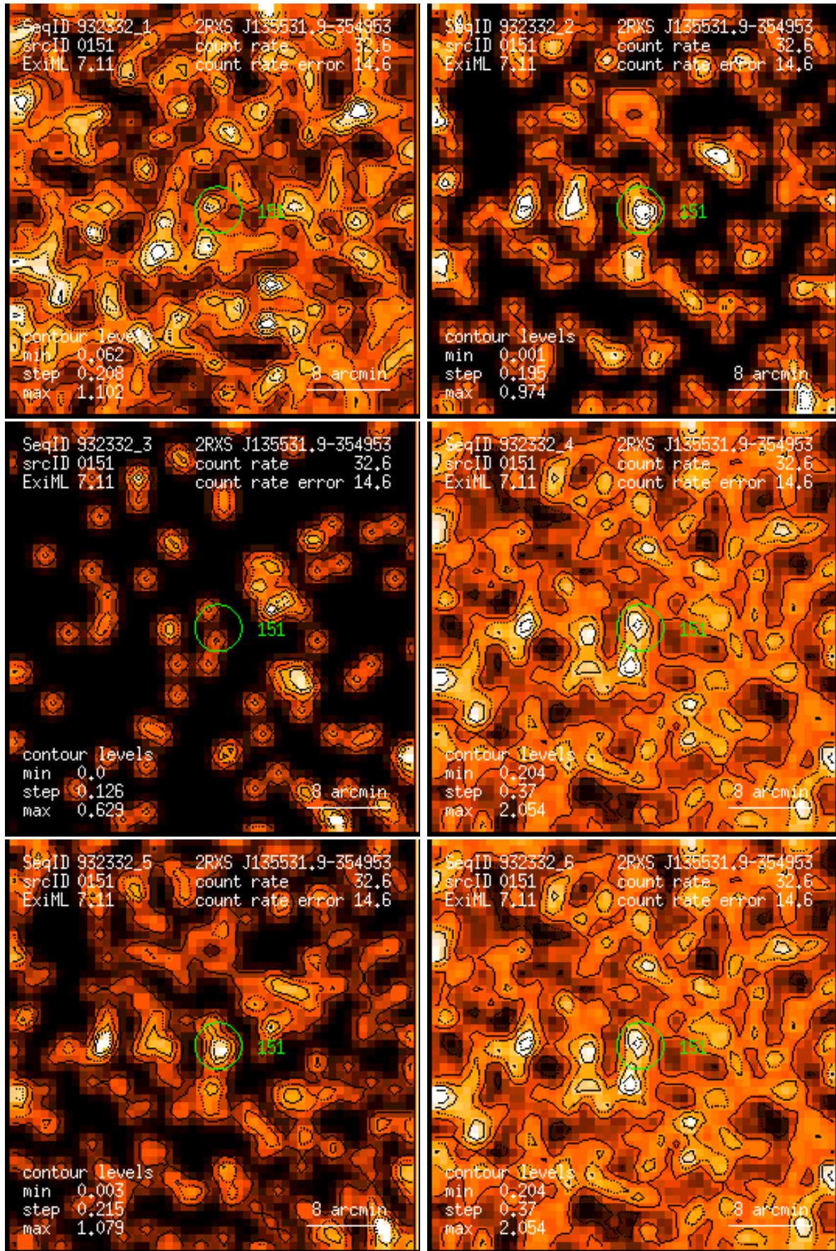
Figure 151: RASS 932332: detection 0151: band rate images, Gaussian filter: (1) PSPC channels 11 – 41, (2) 52 – 90, (3) 91 – 201, (4) 11 – 235, (5) 52 – 201, (6) 11 – 201. Broad band rates in counts/ks. Band rate contour levels in counts/ks/arcmin 2 .
