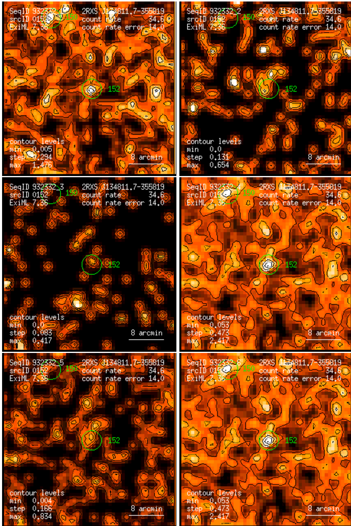
Figure 152: RASS 932332: detection 0152: band rate images, Gaussian filter: (1) PSPC channels 11 – 41, (2) 52 – 90, (3) 91 – 201, (4) 11 – 235, (5) 52 – 201, (6) 11 – 201. Broad band rates in counts/ks. Band rate contour levels in counts/ks/arcmin 2 .
