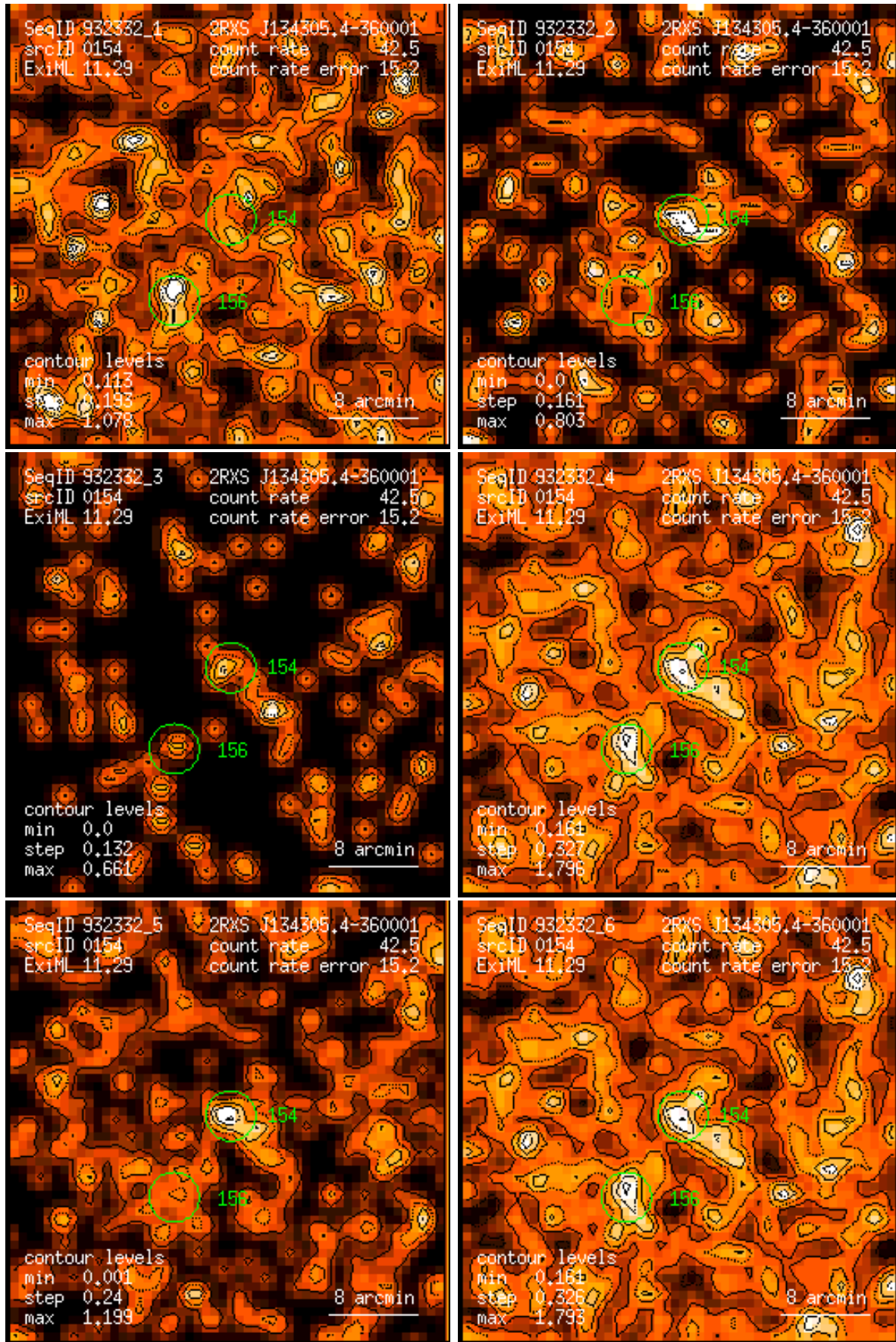
Figure 154: RASS 932332: detection 0154: band rate images, Gaussian filter: (1) PSPC channels 11 – 41, (2) 52 – 90, (3) 91 – 201, (4) 11 – 235, (5) 52 – 201, (6) 11 – 201. Broad band rates in counts/ks. Band rate contour levels in counts/ks/arcmin 2 .
