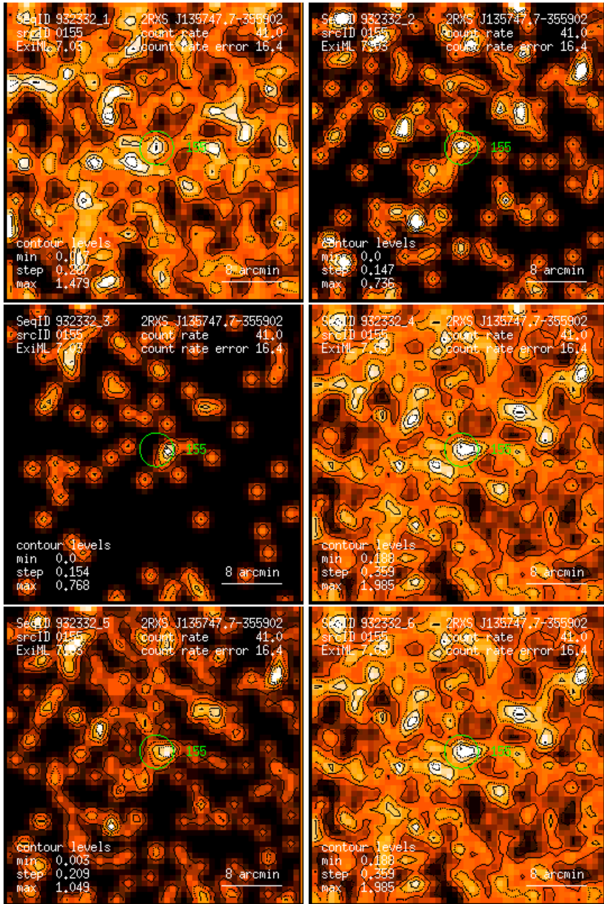
Figure 155: RASS 932332: detection 0155: band rate images, Gaussian filter: (1) PSPC channels 11 – 41, (2) 52 – 90, (3) 91 – 201, (4) 11 – 235, (5) 52 – 201, (6) 11 – 201. Broad band rates in counts/ks. Band rate contour levels in counts/ks/arcmin 2 .
