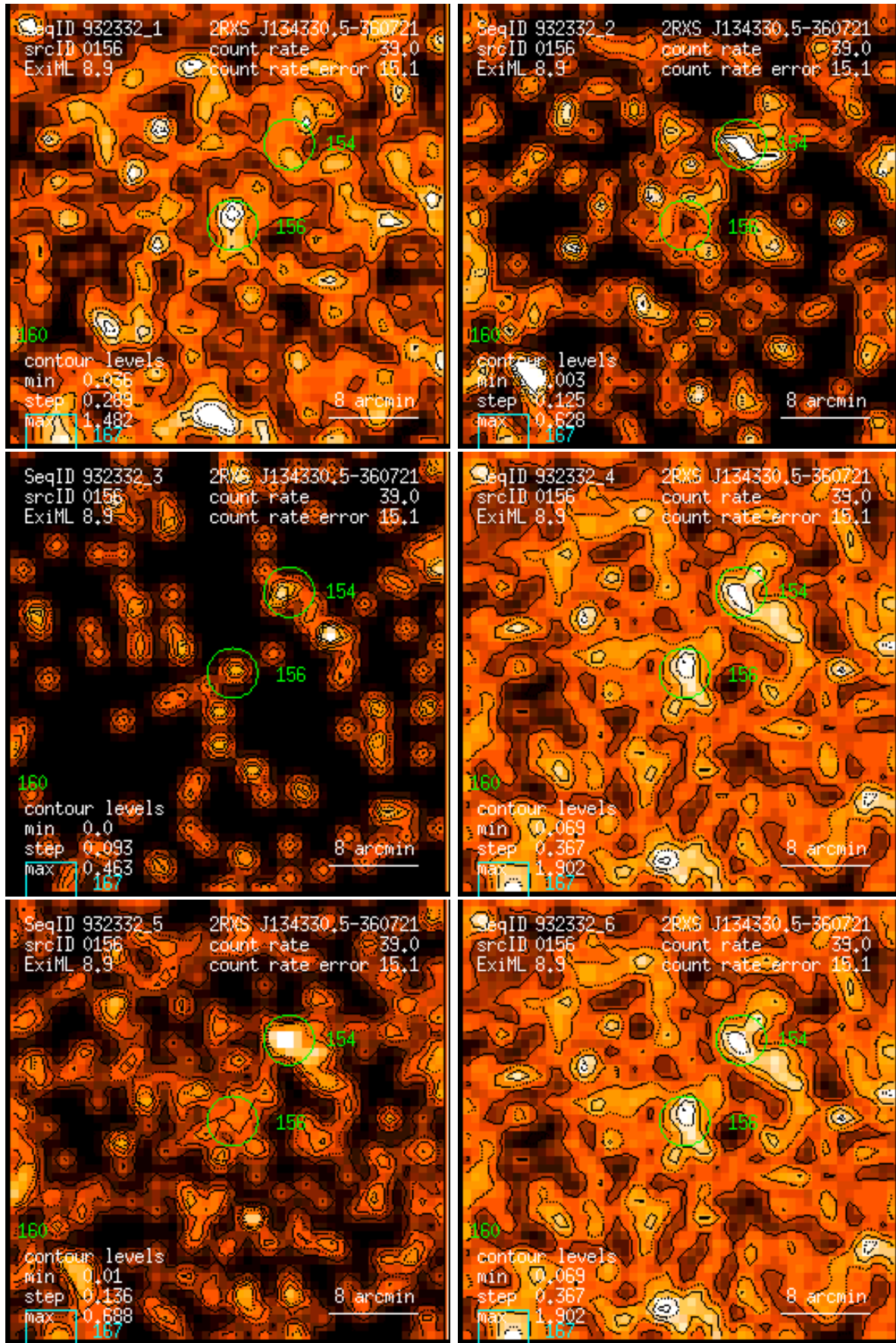
Figure 156: RASS 932332: detection 0156: band rate images, Gaussian filter: (1) PSPC channels 11 – 41, (2) 52 – 90, (3) 91 – 201, (4) 11 – 235, (5) 52 – 201, (6) 11 – 201. Broad band rates in counts/ks. Band rate contour levels in counts/ks/arcmin 2 .
