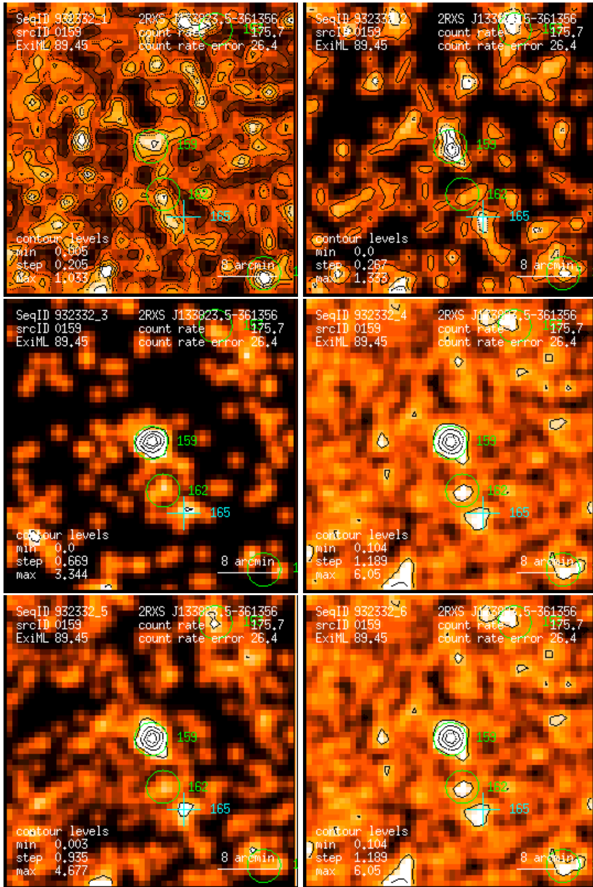
Figure 159: RASS 932332: detection 0159: band rate images, Gaussian filter: (1) PSPC channels 11 – 41, (2) 52 – 90, (3) 91 – 201, (4) 11 – 235, (5) 52 – 201, (6) 11 – 201. Broad band rates in counts/ks. Band rate contour levels in counts/ks/arcmin 2 .
