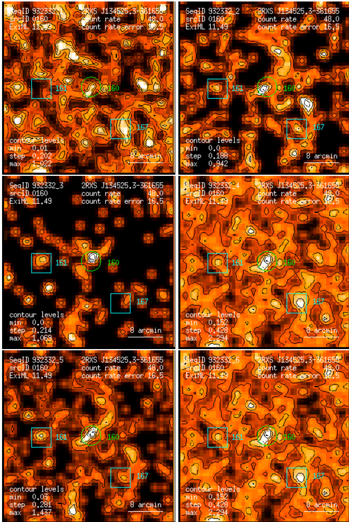
Figure 160: RASS 932332: detection 0160: band rate images, Gaussian filter: (1) PSPC channels 11 – 41, (2) 52 – 90, (3) 91 – 201, (4) 11 – 235, (5) 52 – 201, (6) 11 – 201. Broad band rates in counts/ks. Band rate contour levels in counts/ks/arcmin 2 .
