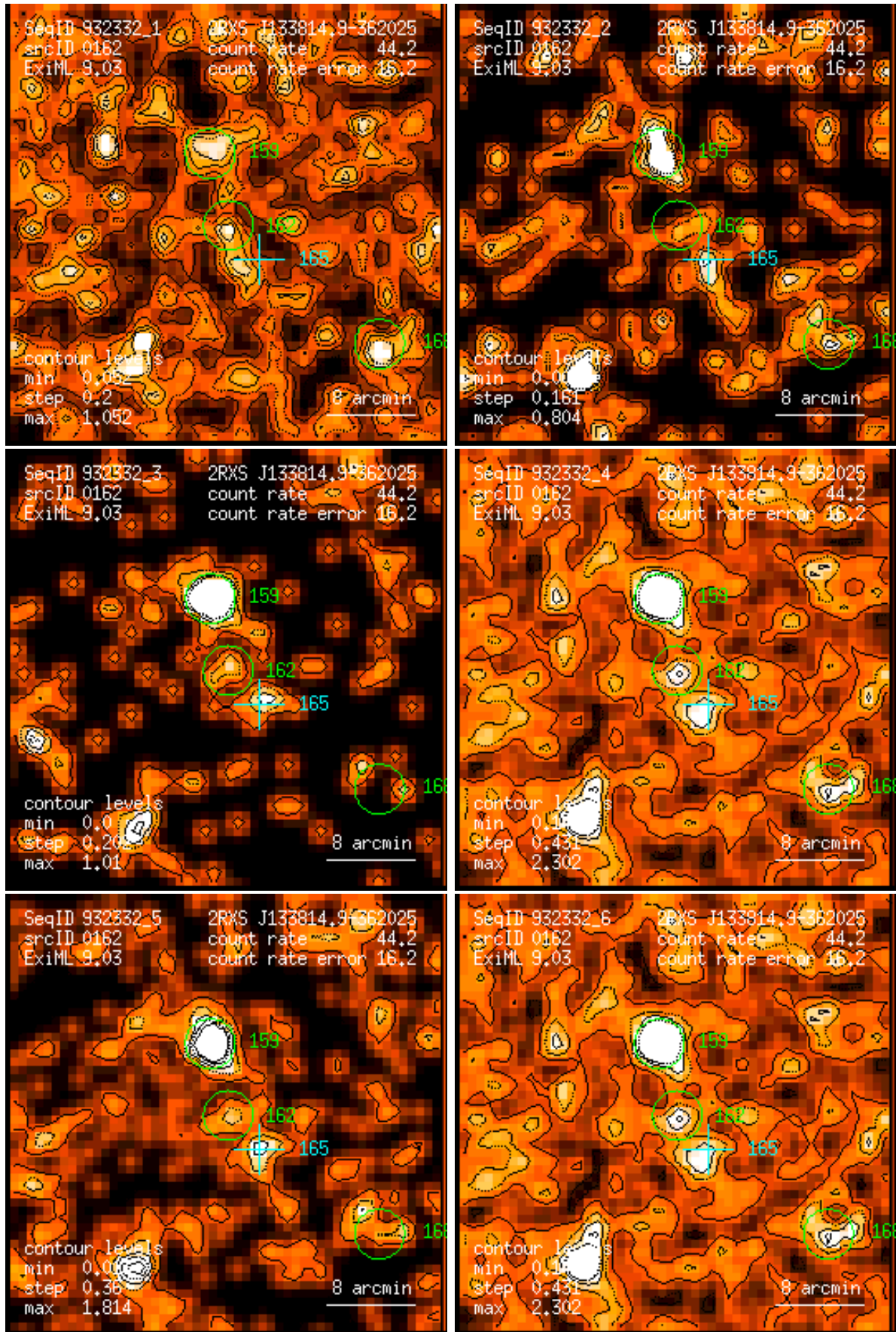
Figure 162: RASS 932332: detection 0162: band rate images, Gaussian filter: (1) PSPC channels 11 – 41, (2) 52 – 90, (3) 91 – 201, (4) 11 – 235, (5) 52 – 201, (6) 11 – 201. Broad band rates in counts/ks. Band rate contour levels in counts/ks/arcmin 2 .
