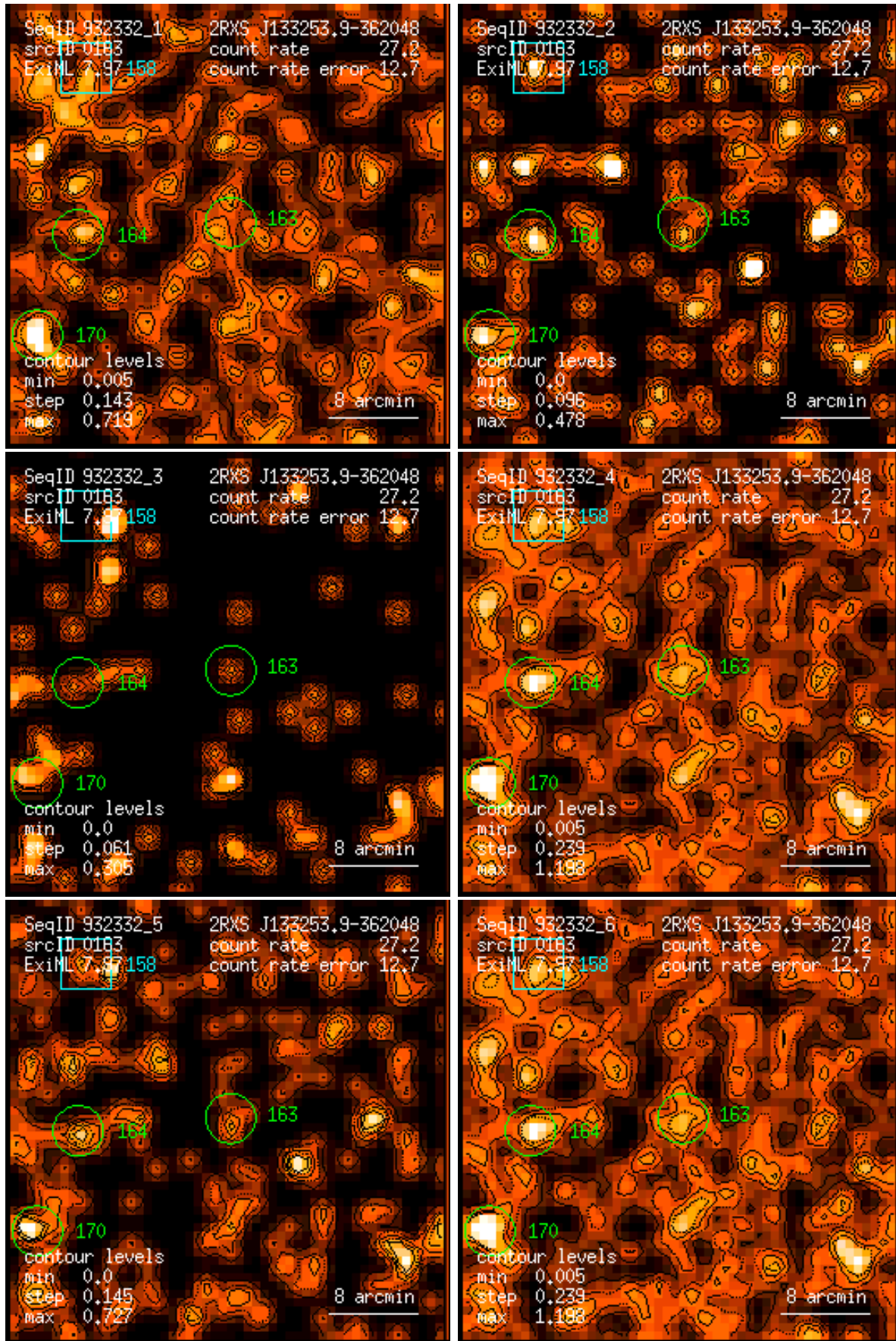
Figure 163: RASS 932332: detection 0163: band rate images, Gaussian filter: (1) PSPC channels 11 – 41, (2) 52 – 90, (3) 91 – 201, (4) 11 – 235, (5) 52 – 201, (6) 11 – 201. Broad band rates in counts/ks. Band rate contour levels in counts/ks/arcmin 2 .
