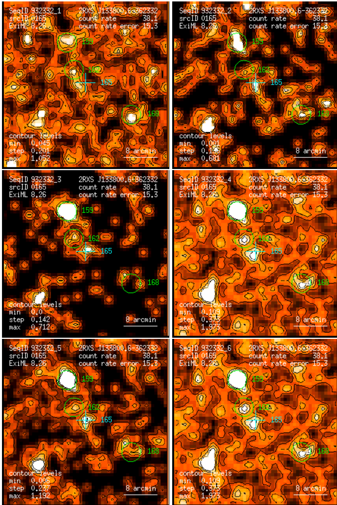
Figure 165: RASS 932332: detection 0165: band rate images, Gaussian filter: (1) PSPC channels 11 – 41, (2) 52 – 90, (3) 91 – 201, (4) 11 – 235, (5) 52 – 201, (6) 11 – 201. Broad band rates in counts/ks. Band rate contour levels in counts/ks/arcmin 2 .
