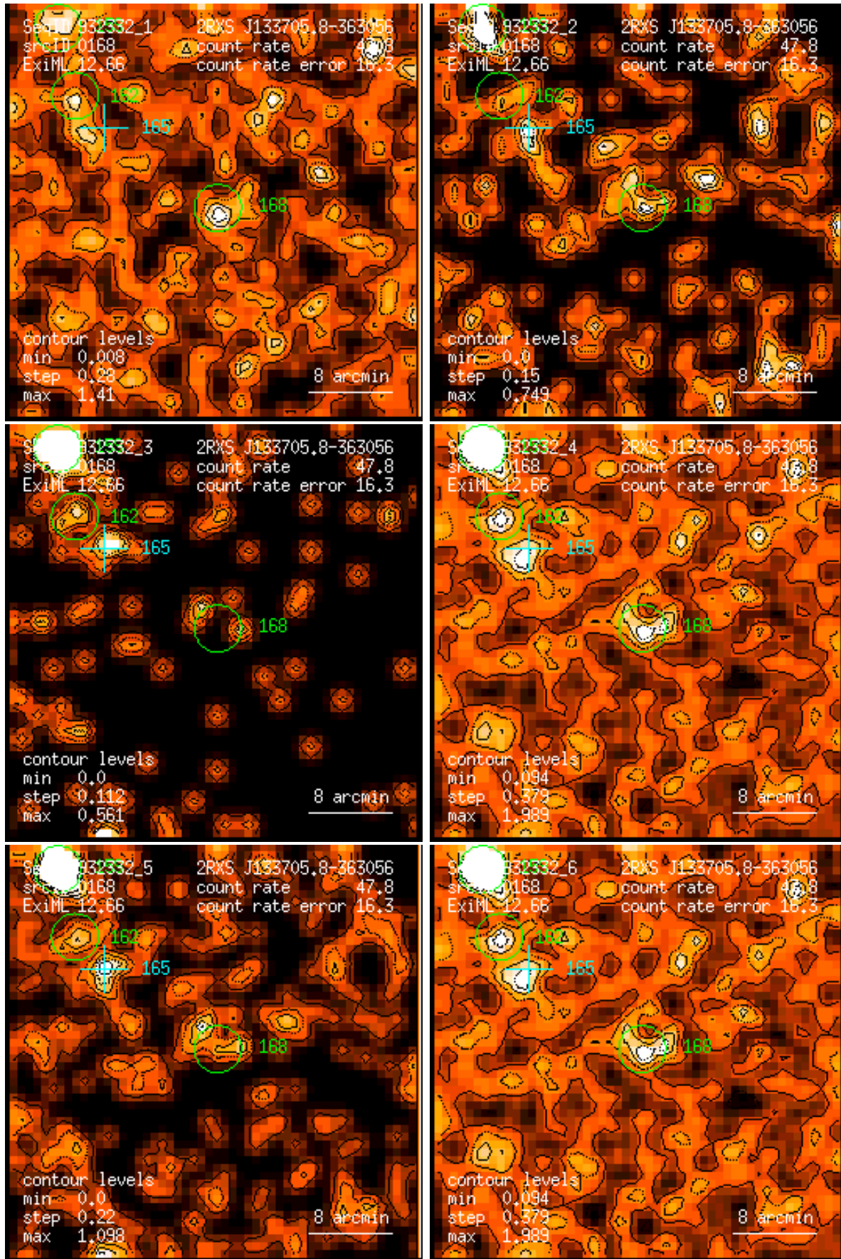
Figure 168: RASS 932332: detection 0168: band rate images, Gaussian filter: (1) PSPC channels 11 – 41, (2) 52 – 90, (3) 91 – 201, (4) 11 – 235, (5) 52 – 201, (6) 11 – 201. Broad band rates in counts/ks. Band rate contour levels in counts/ks/arcmin 2 .
