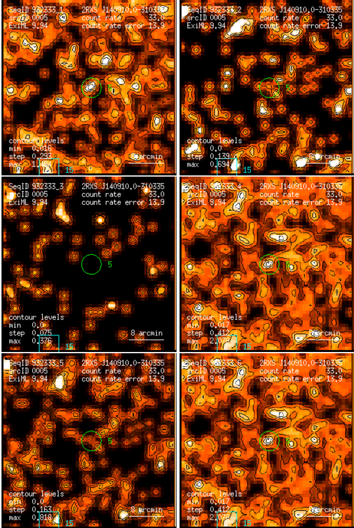
Figure 5: RASS 932333: detection 0005: band rate images, Gaussian filter: (1) PSPC channels 11 – 41, (2) 52 – 90, (3) 91 – 201, (4) 11 – 235, (5) 52 – 201, (6) 11 – 201. Broad band rates in counts/ks. Band rate contour levels in counts/ks/arcmin 2 .
