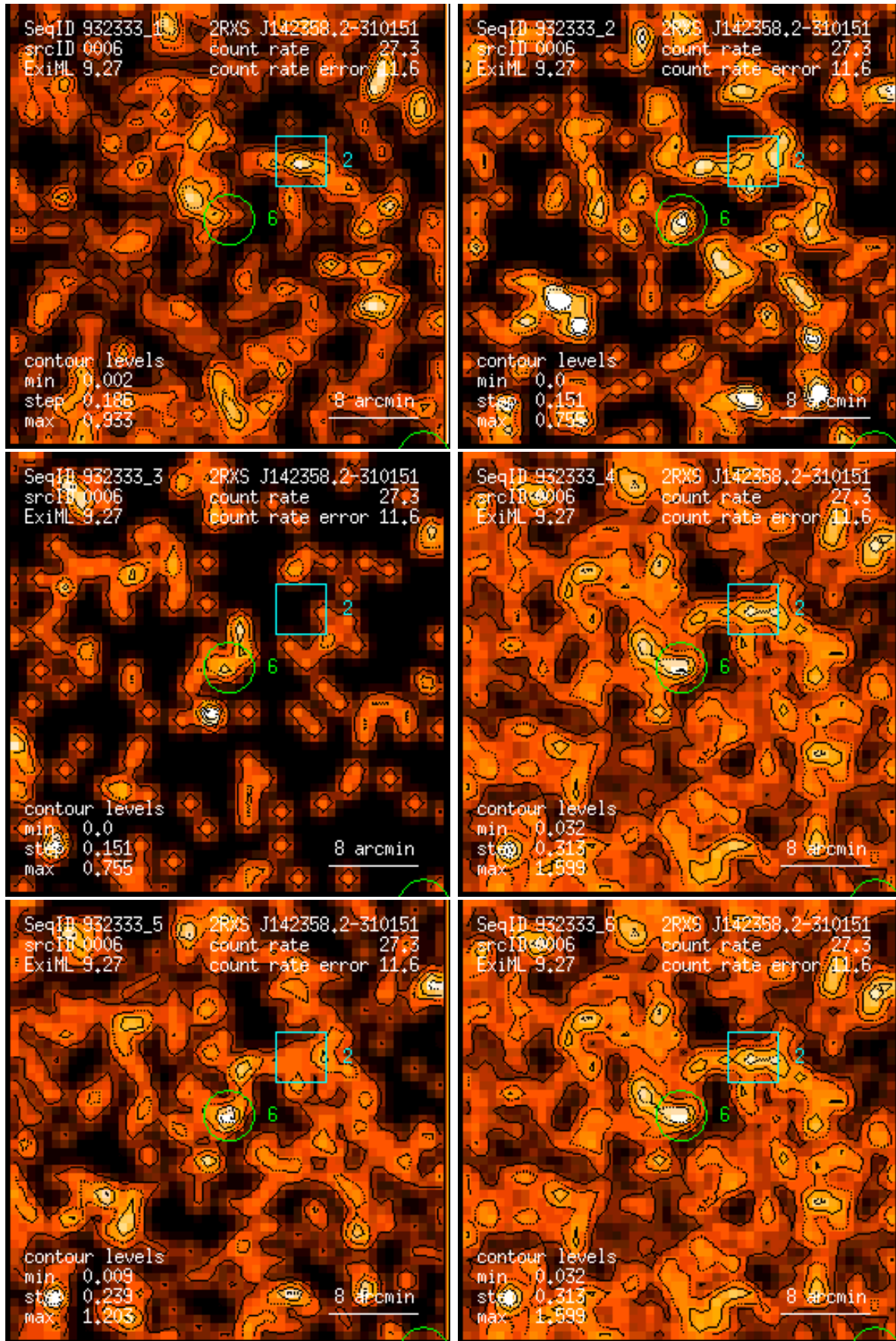
Figure 6: RASS 932333: detection 0006: band rate images, Gaussian filter: (1) PSPC channels 11 – 41, (2) 52 – 90, (3) 91 – 201, (4) 11 – 235, (5) 52 – 201, (6) 11 – 201. Broad band rates in counts/ks. Band rate contour levels in counts/ks/arcmin 2 .
