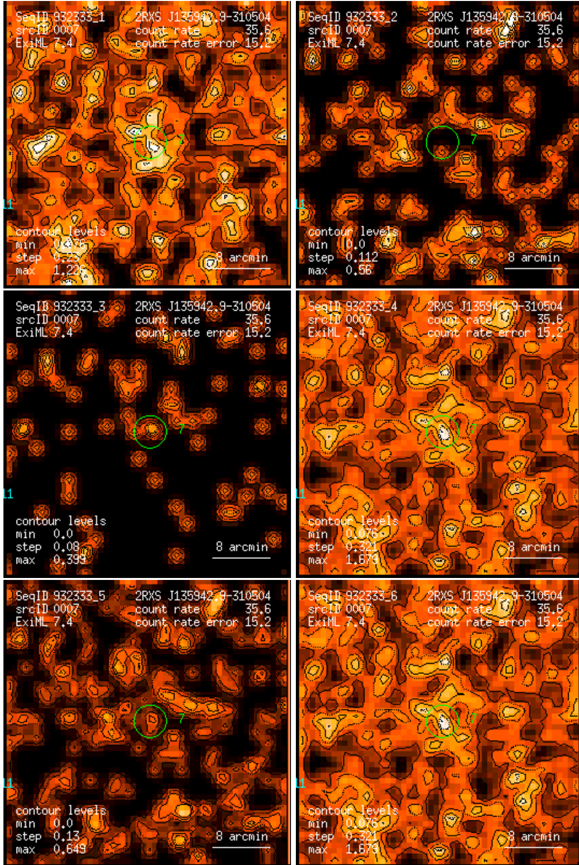
Figure 7: RASS 932333: detection 0007: band rate images, Gaussian filter: (1) PSPC channels 11 – 41, (2) 52 – 90, (3) 91 – 201, (4) 11 – 235, (5) 52 – 201, (6) 11 – 201. Broad band rates in counts/ks. Band rate contour levels in counts/ks/arcmin 2 .
