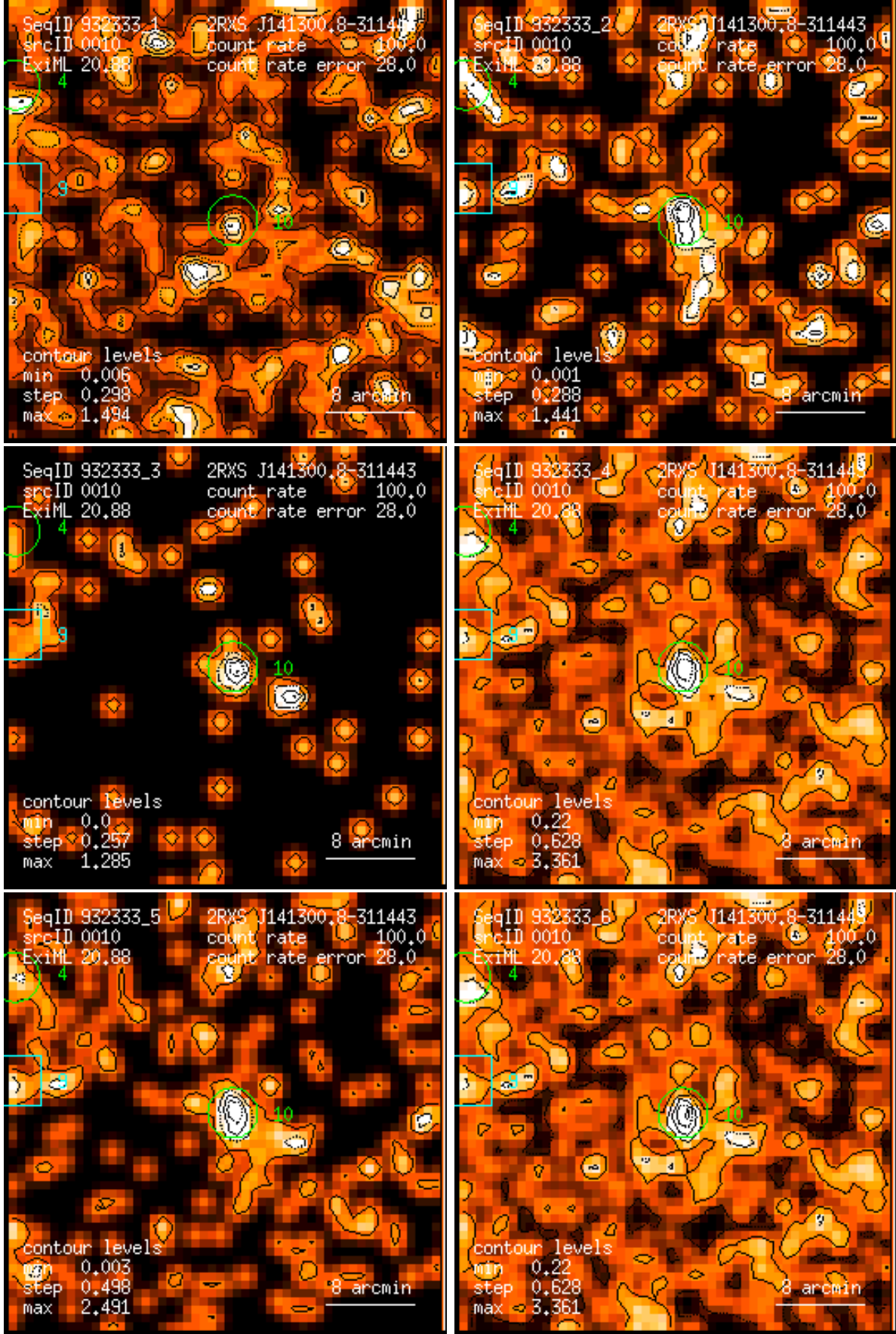
Figure 10: RASS 932333: detection 0010: band rate images, Gaussian filter: (1) PSPC channels 11 – 41, (2) 52 – 90, (3) 91 – 201, (4) 11 – 235, (5) 52 – 201, (6) 11 – 201. Broad band rates in counts/ks. Band rate contour levels in counts/ks/arcmin 2 .
